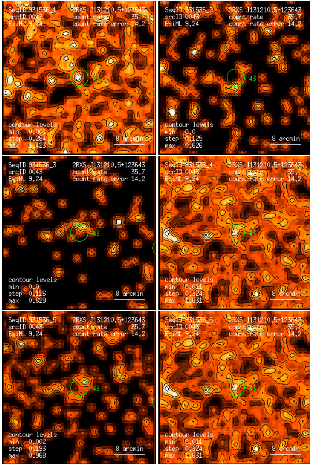
Figure 43: RASS 931536: detection 0043: band rate images, Gaussian filter: (1) PSPC channels 11 – 41, (2) 52 – 90, (3) 91 – 201, (4) 11 – 235, (5) 52 – 201, (6) 11 – 201. Broad band rates in counts/ks. Band rate contour levels in counts/ks/arcmin 2 .
