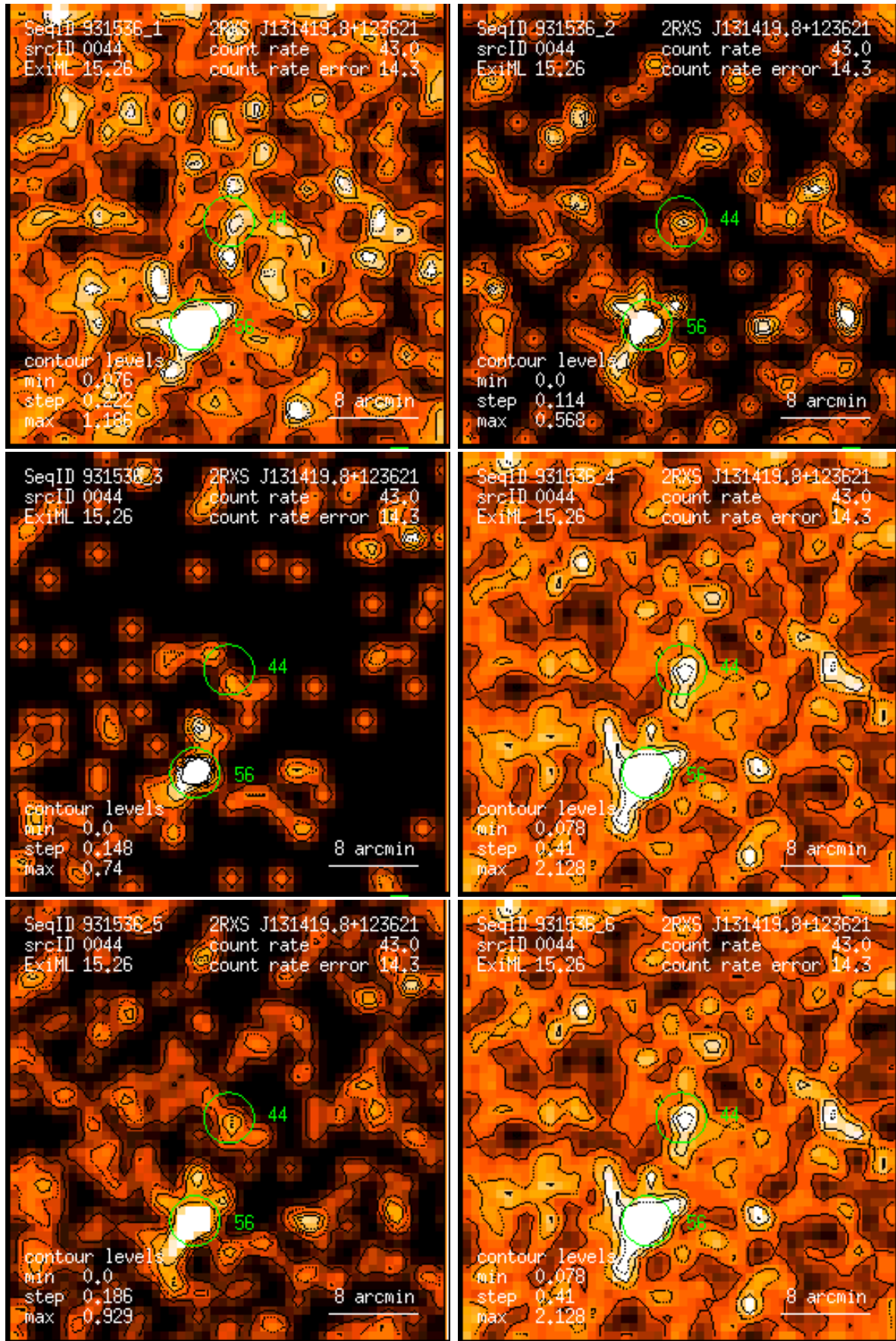
Figure 44: RASS 931536: detection 0044: band rate images, Gaussian filter: (1) PSPC channels 11 – 41, (2) 52 – 90, (3) 91 – 201, (4) 11 – 235, (5) 52 – 201, (6) 11 – 201. Broad band rates in counts/ks. Band rate contour levels in counts/ks/arcmin 2 .
