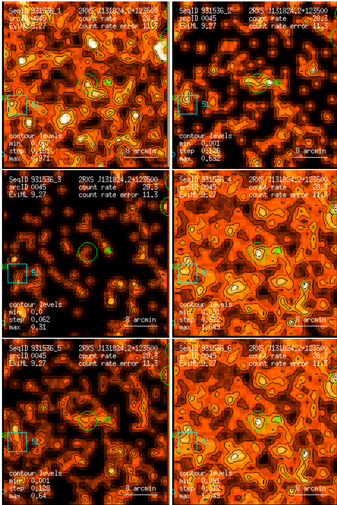
Figure 45: RASS 931536: detection 0045: band rate images, Gaussian filter: (1) PSPC channels 11 – 41, (2) 52 – 90, (3) 91 – 201, (4) 11 – 235, (5) 52 – 201, (6) 11 – 201. Broad band rates in counts/ks. Band rate contour levels in counts/ks/arcmin 2 .
