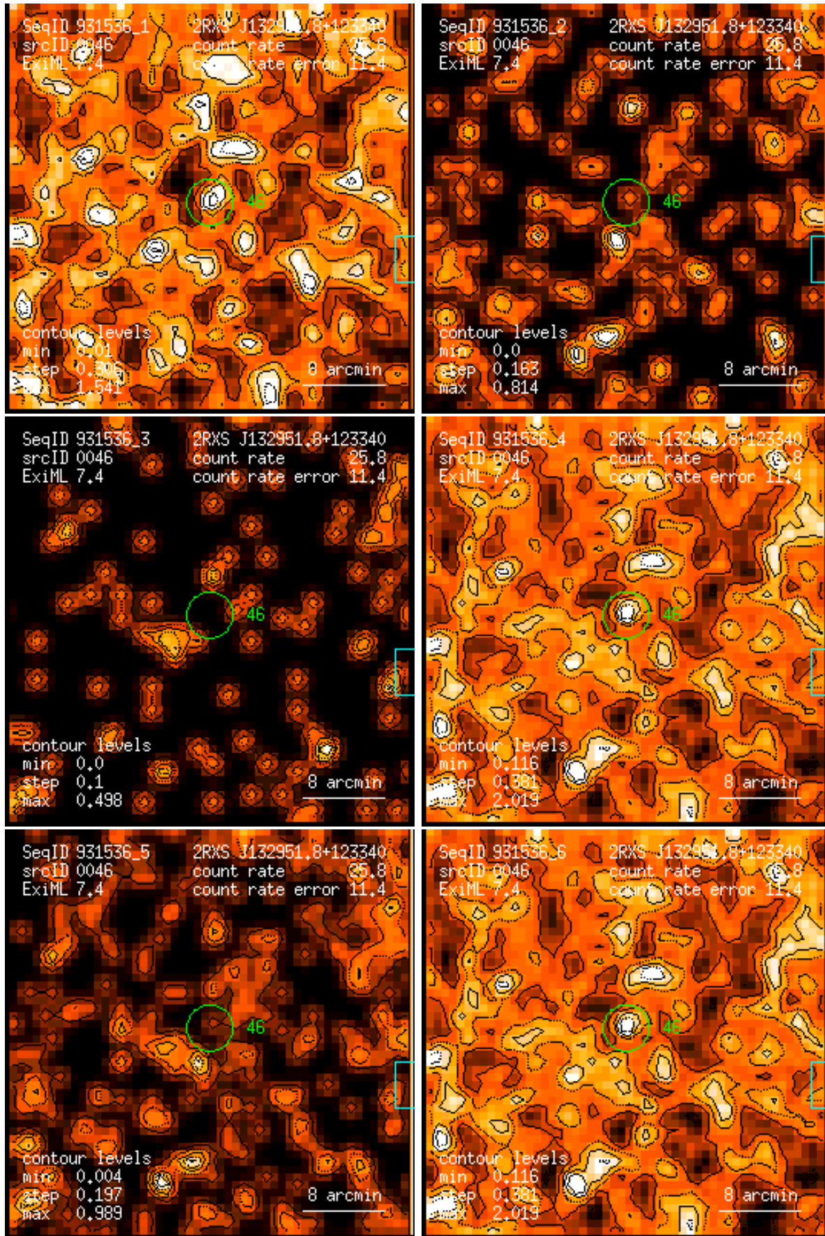
Figure 46: RASS 931536: detection 0046: band rate images, Gaussian filter: (1) PSPC channels 11 – 41, (2) 52 – 90, (3) 91 – 201, (4) 11 – 235, (5) 52 – 201, (6) 11 – 201. Broad band rates in counts/ks. Band rate contour levels in counts/ks/arcmin 2 .
