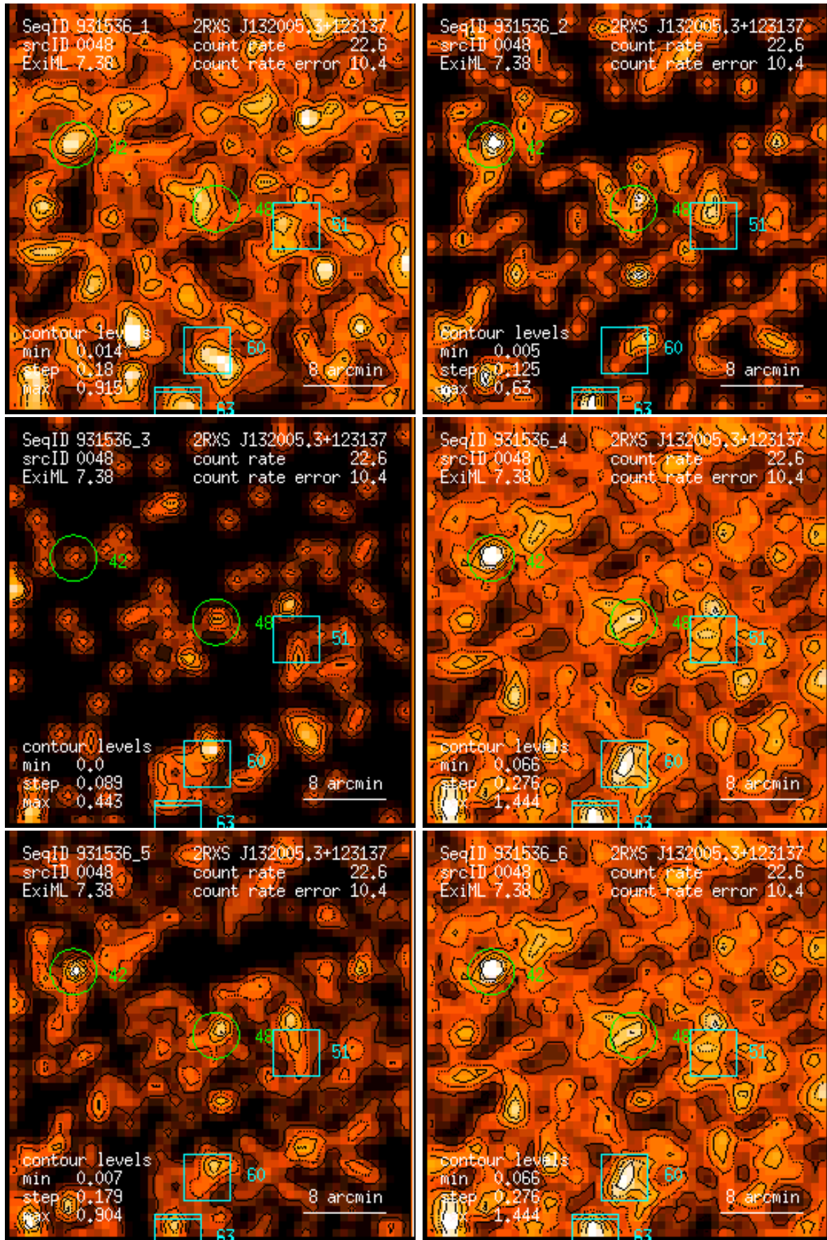
Figure 48: RASS 931536: detection 0048: band rate images, Gaussian filter: (1) PSPC channels 11 – 41, (2) 52 – 90, (3) 91 – 201, (4) 11 – 235, (5) 52 – 201, (6) 11 – 201. Broad band rates in counts/ks. Band rate contour levels in counts/ks/arcmin 2 .
