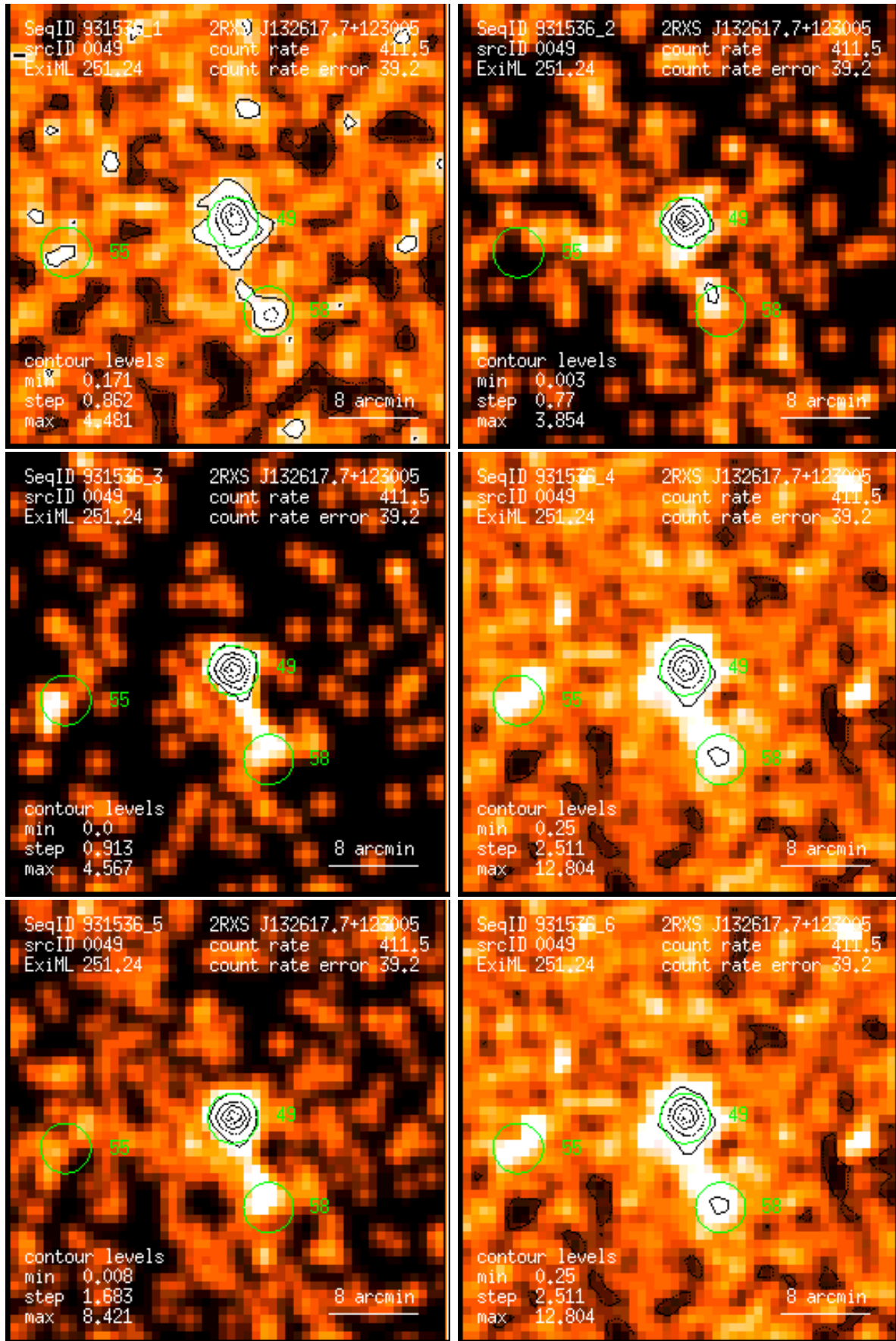
Figure 49: RASS 931536: detection 0049: band rate images, Gaussian filter: (1) PSPC channels 11 – 41, (2) 52 – 90, (3) 91 – 201, (4) 11 – 235, (5) 52 – 201, (6) 11 – 201. Broad band rates in counts/ks. Band rate contour levels in counts/ks/arcmin 2 .
