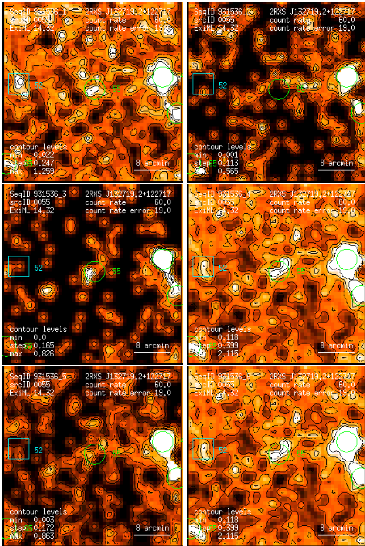
Figure 55: RASS 931536: detection 0055: band rate images, Gaussian filter: (1) PSPC channels 11 – 41, (2) 52 – 90, (3) 91 – 201, (4) 11 – 235, (5) 52 – 201, (6) 11 – 201. Broad band rates in counts/ks. Band rate contour levels in counts/ks/arcmin 2 .
