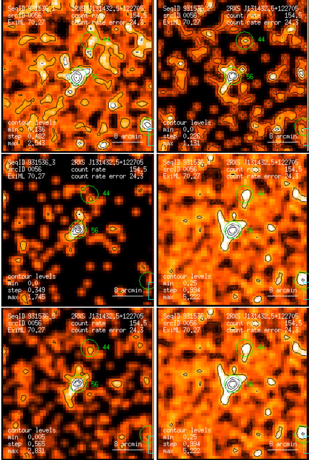
Figure 56: RASS 931536: detection 0056: band rate images, Gaussian filter: (1) PSPC channels 11 – 41, (2) 52 – 90, (3) 91 – 201, (4) 11 – 235, (5) 52 – 201, (6) 11 – 201. Broad band rates in counts/ks. Band rate contour levels in counts/ks/arcmin 2 .
