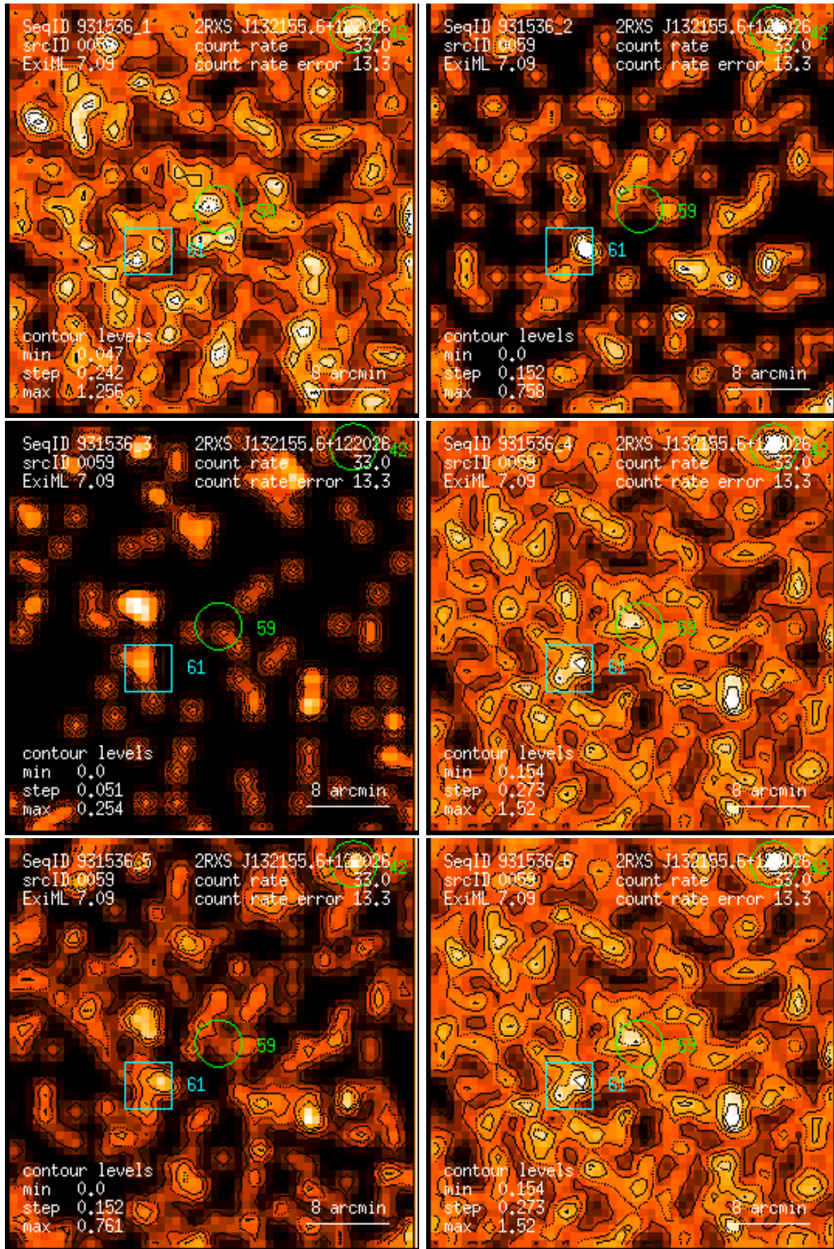
Figure 59: RASS 931536: detection 0059: band rate images, Gaussian filter: (1) PSPC channels 11 – 41, (2) 52 – 90, (3) 91 – 201, (4) 11 – 235, (5) 52 – 201, (6) 11 – 201. Broad band rates in counts/ks. Band rate contour levels in counts/ks/arcmin 2 .
