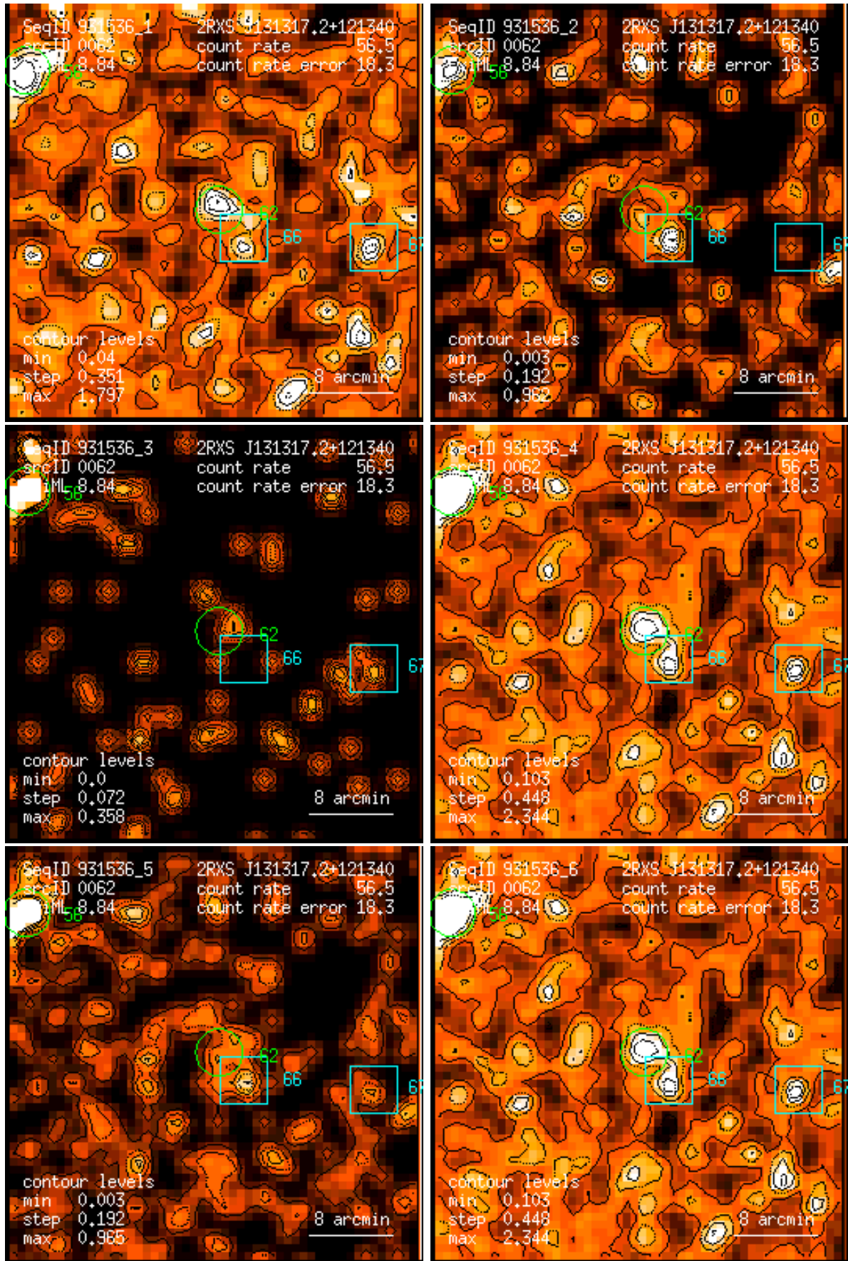
Figure 62: RASS 931536: detection 0062: band rate images, Gaussian filter: (1) PSPC channels 11 – 41, (2) 52 – 90, (3) 91 – 201, (4) 11 – 235, (5) 52 – 201, (6) 11 – 201. Broad band rates in counts/ks. Band rate contour levels in counts/ks/arcmin 2 .
