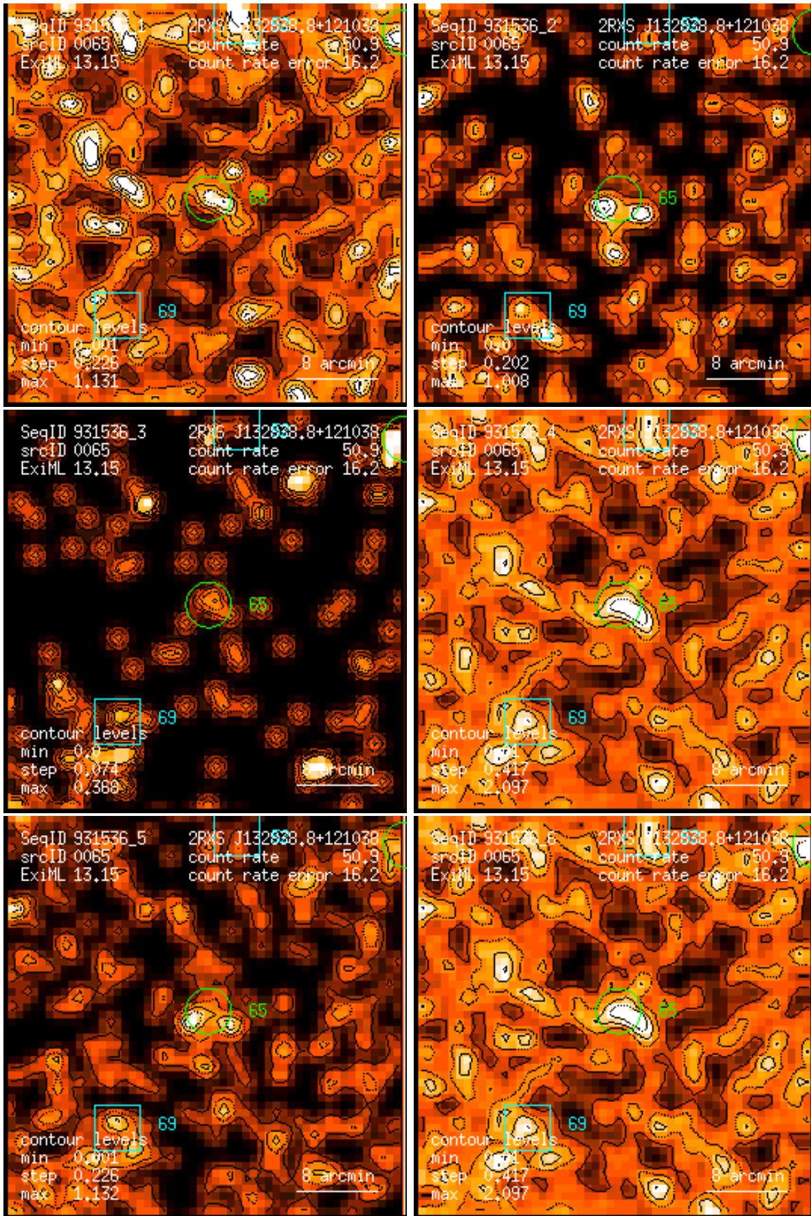
Figure 65: RASS 931536: detection 0065: band rate images, Gaussian filter: (1) PSPC channels 11 – 41, (2) 52 – 90, (3) 91 – 201, (4) 11 – 235, (5) 52 – 201, (6) 11 – 201. Broad band rates in counts/ks. Band rate contour levels in counts/ks/arcmin 2 .
