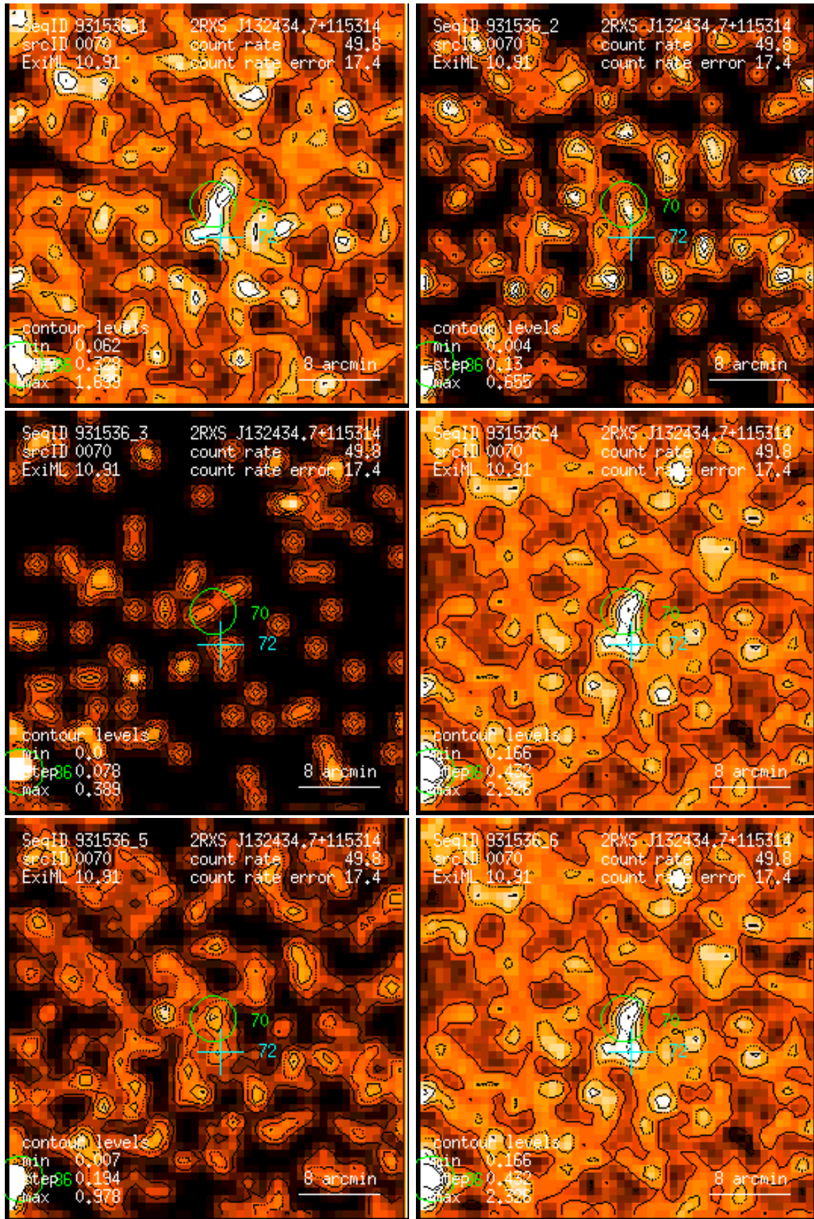
Figure 70: RASS 931536: detection 0070: band rate images, Gaussian filter: (1) PSPC channels 11 – 41, (2) 52 – 90, (3) 91 – 201, (4) 11 – 235, (5) 52 – 201, (6) 11 – 201. Broad band rates in counts/ks. Band rate contour levels in counts/ks/arcmin 2 .
