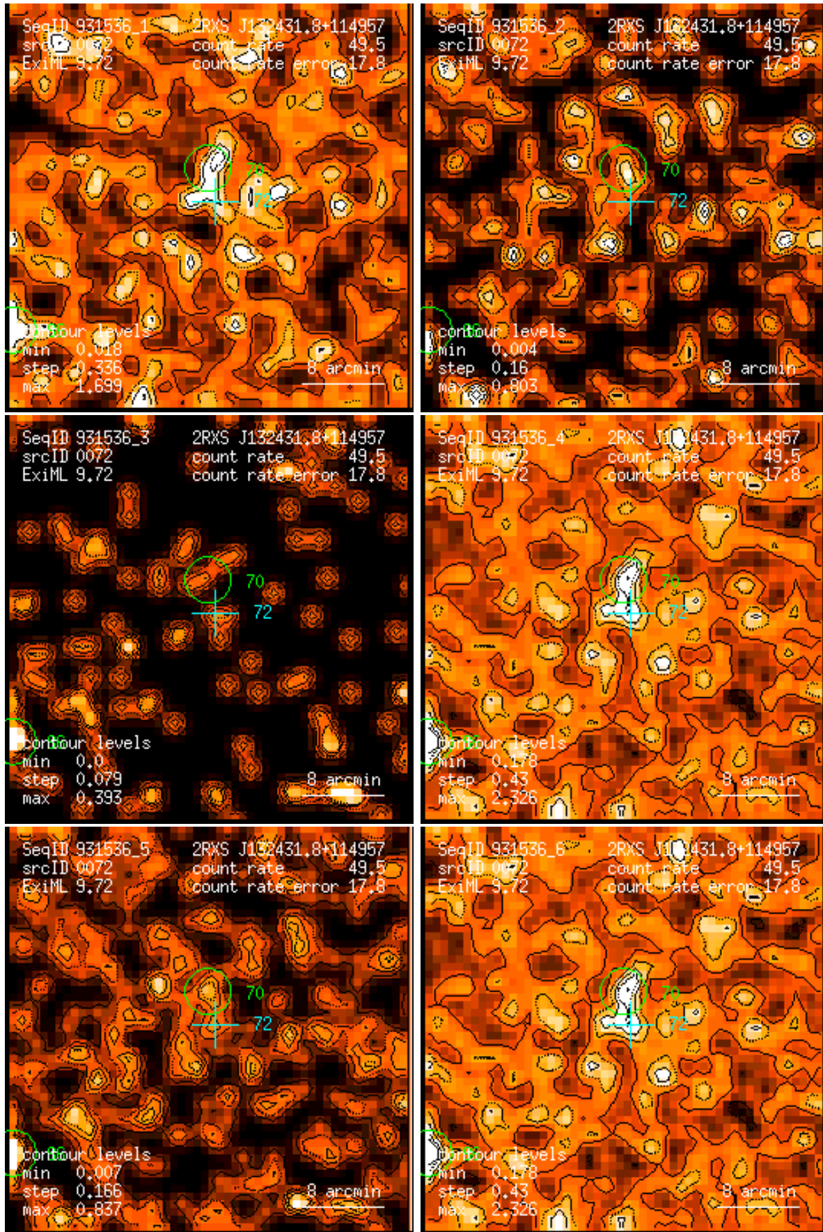
Figure 72: RASS 931536: detection 0072: band rate images, Gaussian filter: (1) PSPC channels 11 – 41, (2) 52 – 90, (3) 91 – 201, (4) 11 – 235, (5) 52 – 201, (6) 11 – 201. Broad band rates in counts/ks. Band rate contour levels in counts/ks/arcmin 2 .
