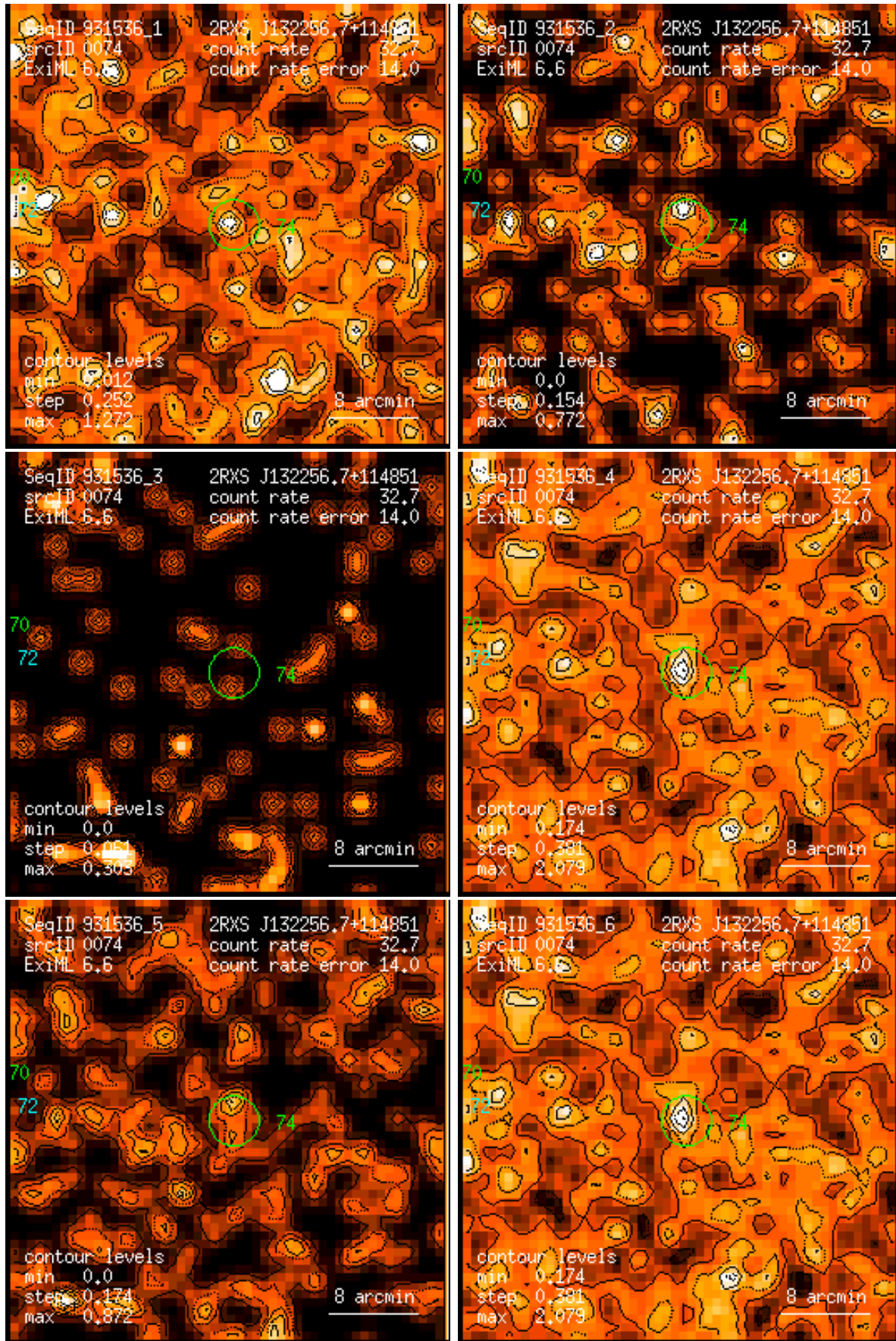
Figure 74: RASS 931536: detection 0074: band rate images, Gaussian filter: (1) PSPC channels 11 – 41, (2) 52 – 90, (3) 91 – 201, (4) 11 – 235, (5) 52 – 201, (6) 11 – 201. Broad band rates in counts/ks. Band rate contour levels in counts/ks/arcmin 2 .
