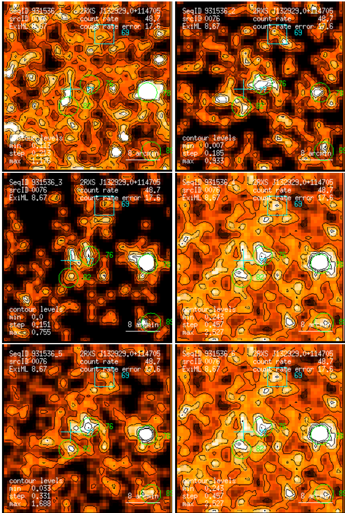
Figure 76: RASS 931536: detection 0076: band rate images, Gaussian filter: (1) PSPC channels 11 – 41, (2) 52 – 90, (3) 91 – 201, (4) 11 – 235, (5) 52 – 201, (6) 11 – 201. Broad band rates in counts/ks. Band rate contour levels in counts/ks/arcmin 2 .
