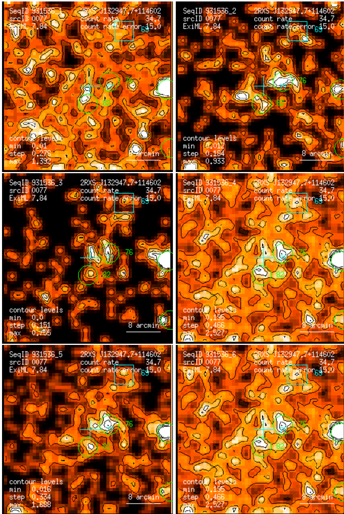
Figure 77: RASS 931536: detection 0077: band rate images, Gaussian filter: (1) PSPC channels 11 – 41, (2) 52 – 90, (3) 91 – 201, (4) 11 – 235, (5) 52 – 201, (6) 11 – 201. Broad band rates in counts/ks. Band rate contour levels in counts/ks/arcmin 2 .
