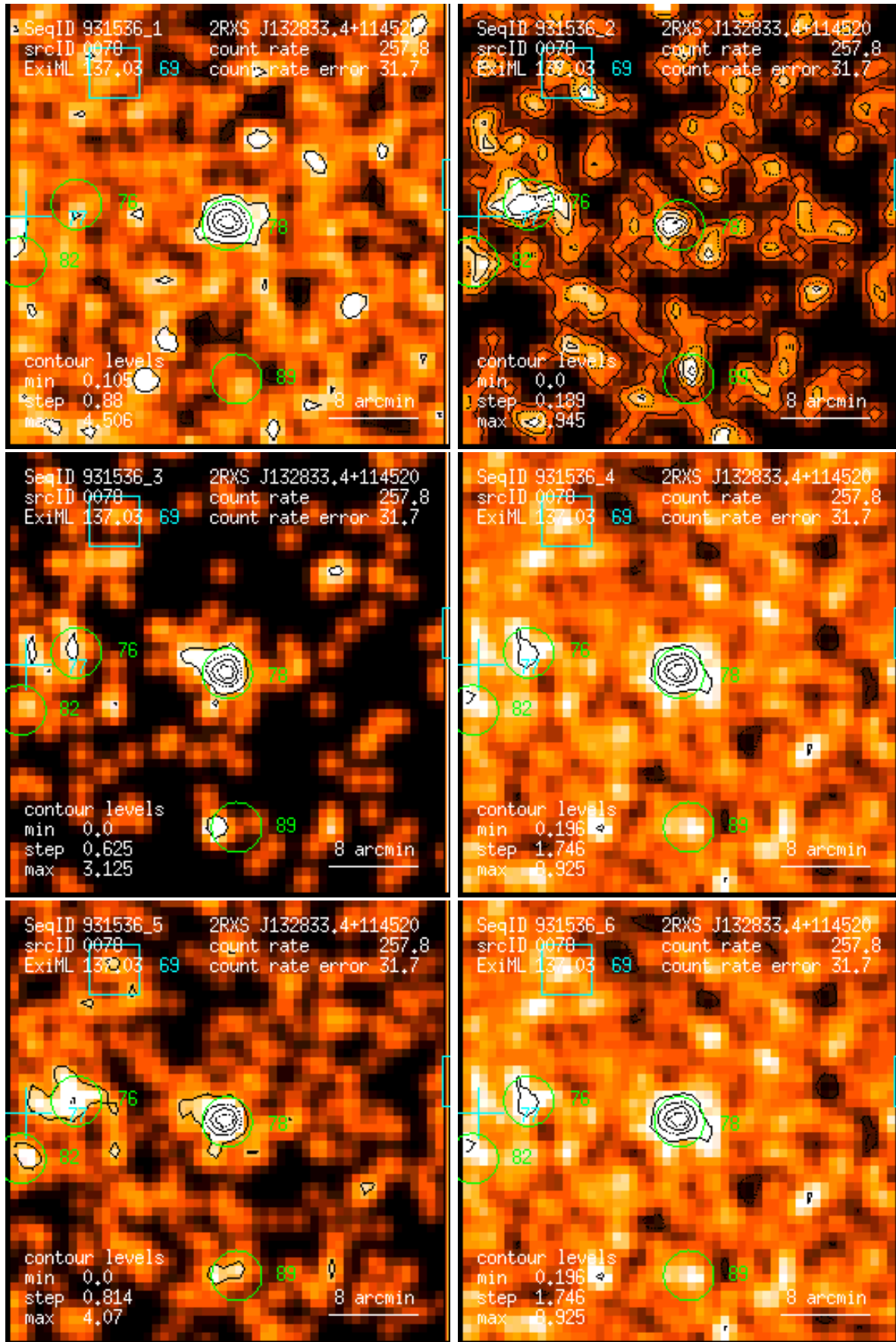
Figure 78: RASS 931536: detection 0078: band rate images, Gaussian filter: (1) PSPC channels 11 – 41, (2) 52 – 90, (3) 91 – 201, (4) 11 – 235, (5) 52 – 201, (6) 11 – 201. Broad band rates in counts/ks. Band rate contour levels in counts/ks/arcmin 2 .
