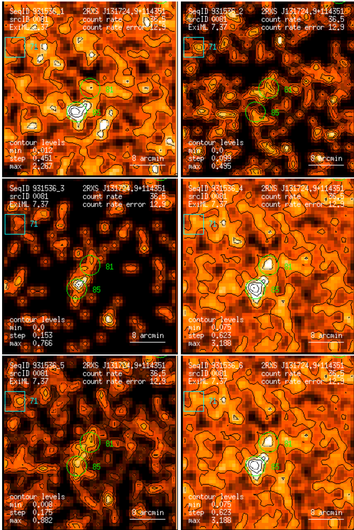
Figure 81: RASS 931536: detection 0081: band rate images, Gaussian filter: (1) PSPC channels 11 – 41, (2) 52 – 90, (3) 91 – 201, (4) 11 – 235, (5) 52 – 201, (6) 11 – 201. Broad band rates in counts/ks. Band rate contour levels in counts/ks/arcmin 2 .
