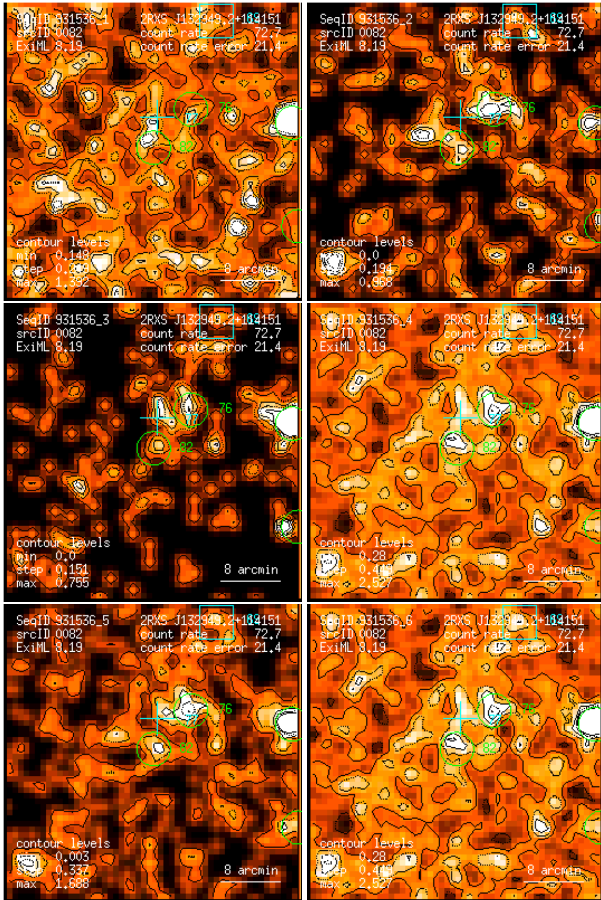
Figure 82: RASS 931536: detection 0082: band rate images, Gaussian filter: (1) PSPC channels 11 – 41, (2) 52 – 90, (3) 91 – 201, (4) 11 – 235, (5) 52 – 201, (6) 11 – 201. Broad band rates in counts/ks. Band rate contour levels in counts/ks/arcmin 2 .
