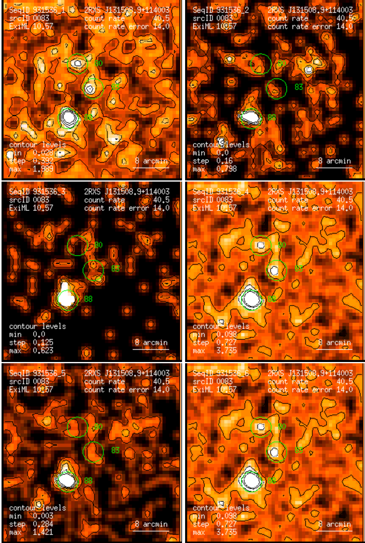
Figure 83: RASS 931536: detection 0083: band rate images, Gaussian filter: (1) PSPC channels 11 – 41, (2) 52 – 90, (3) 91 – 201, (4) 11 – 235, (5) 52 – 201, (6) 11 – 201. Broad band rates in counts/ks. Band rate contour levels in counts/ks/arcmin 2 .
