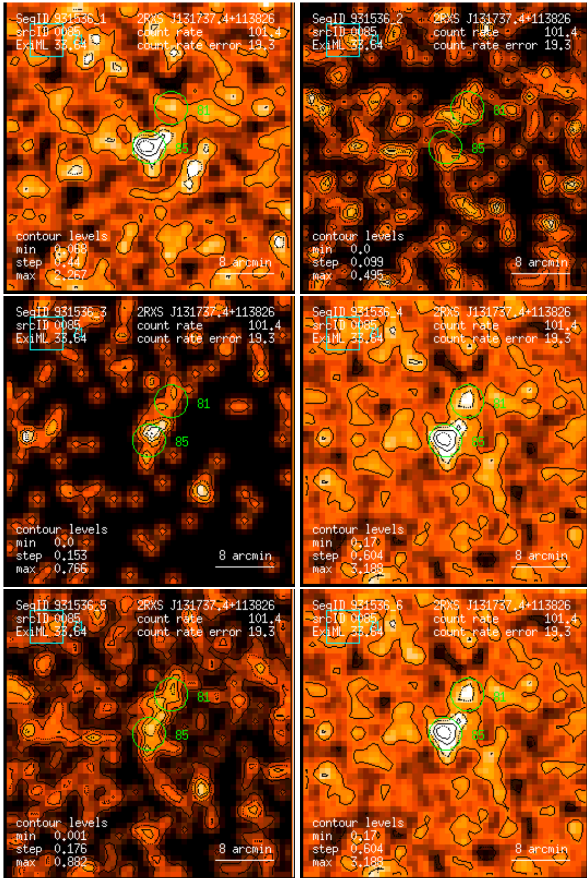
Figure 85: RASS 931536: detection 0085: band rate images, Gaussian filter: (1) PSPC channels 11 – 41, (2) 52 – 90, (3) 91 – 201, (4) 11 – 235, (5) 52 – 201, (6) 11 – 201. Broad band rates in counts/ks. Band rate contour levels in counts/ks/arcmin 2 .
