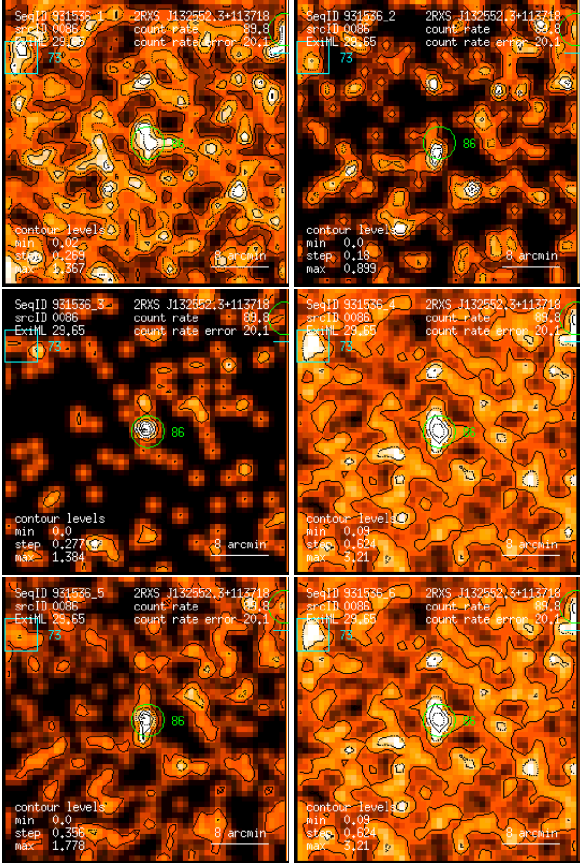
Figure 86: RASS 931536: detection 0086: band rate images, Gaussian filter: (1) PSPC channels 11 – 41, (2) 52 – 90, (3) 91 – 201, (4) 11 – 235, (5) 52 – 201, (6) 11 – 201. Broad band rates in counts/ks. Band rate contour levels in counts/ks/arcmin 2 .
