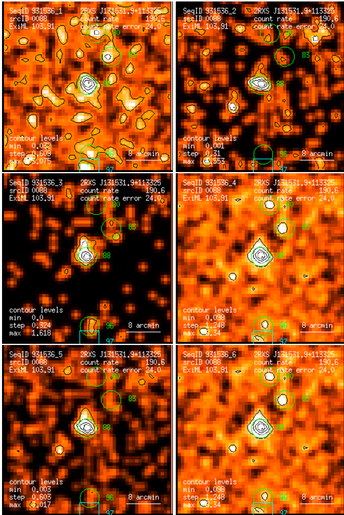
Figure 88: RASS 931536: detection 0088: band rate images, Gaussian filter: (1) PSPC channels 11 – 41, (2) 52 – 90, (3) 91 – 201, (4) 11 – 235, (5) 52 – 201, (6) 11 – 201. Broad band rates in counts/ks. Band rate contour levels in counts/ks/arcmin 2 .
