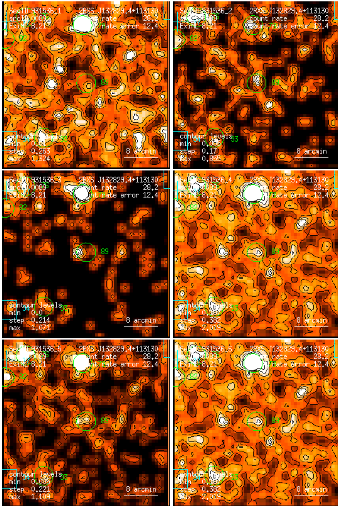
Figure 89: RASS 931536: detection 0089: band rate images, Gaussian filter: (1) PSPC channels 11 – 41, (2) 52 – 90, (3) 91 – 201, (4) 11 – 235, (5) 52 – 201, (6) 11 – 201. Broad band rates in counts/ks. Band rate contour levels in counts/ks/arcmin 2 .
