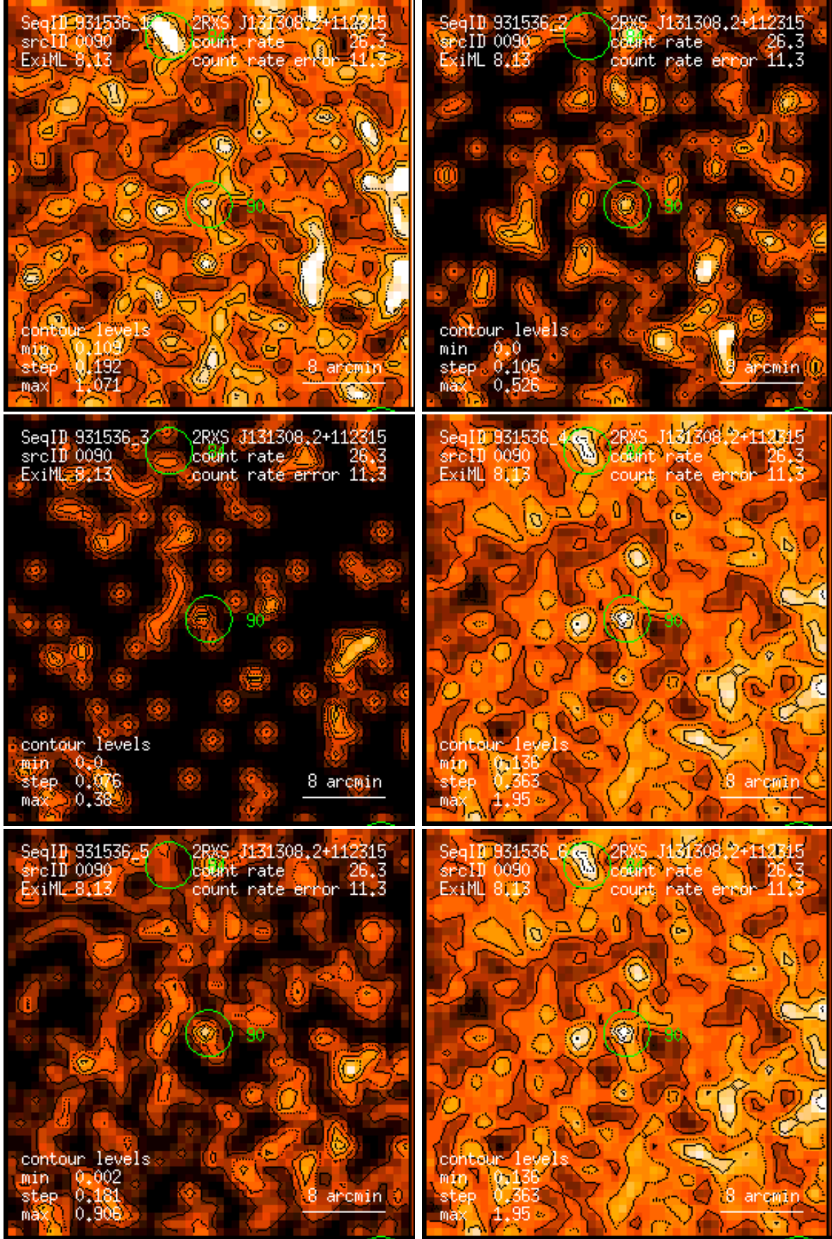
Figure 90: RASS 931536: detection 0090: band rate images, Gaussian filter: (1) PSPC channels 11 – 41, (2) 52 – 90, (3) 91 – 201, (4) 11 – 235, (5) 52 – 201, (6) 11 – 201. Broad band rates in counts/ks. Band rate contour levels in counts/ks/arcmin 2 .
