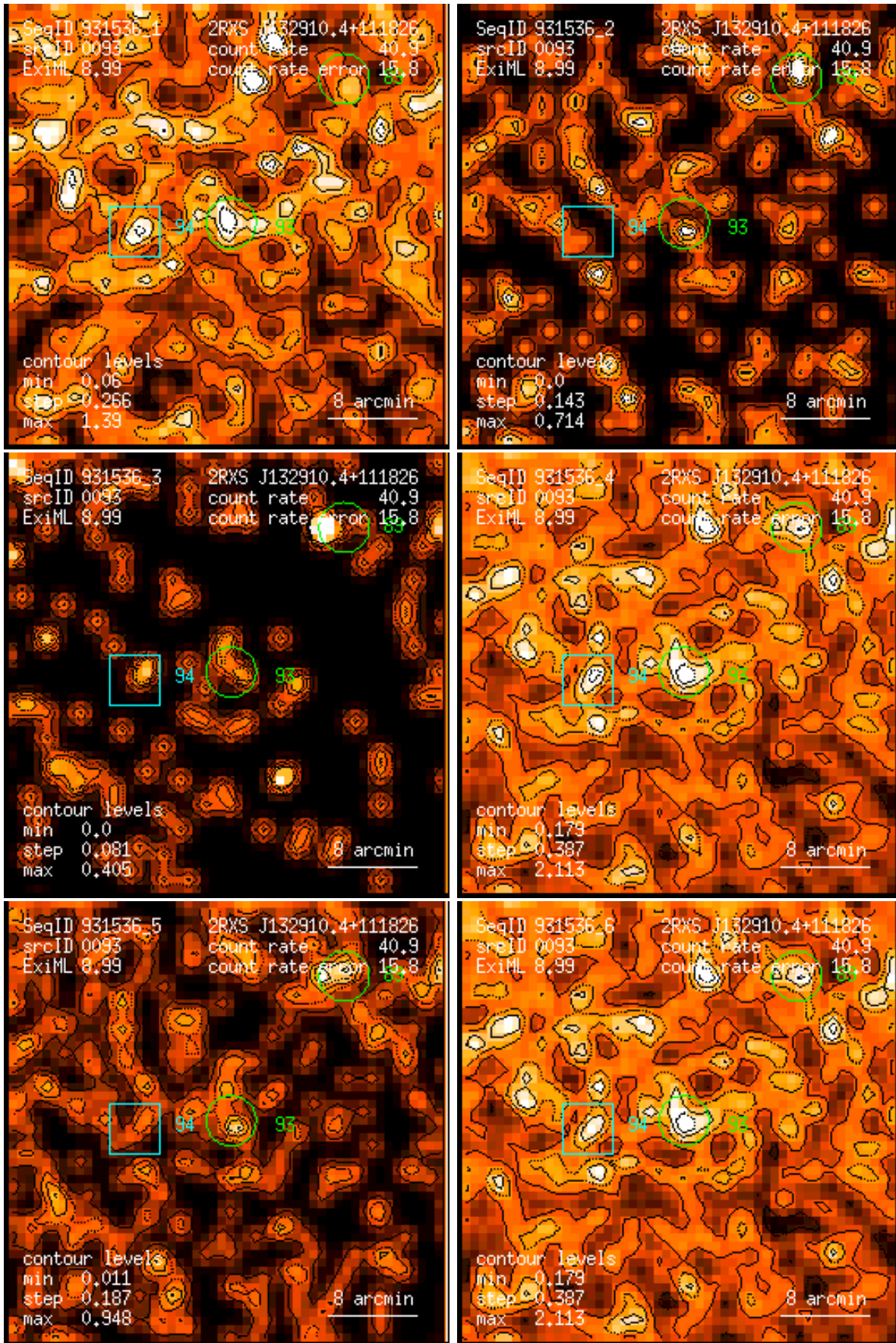
Figure 93: RASS 931536: detection 0093: band rate images, Gaussian filter: (1) PSPC channels 11 – 41, (2) 52 – 90, (3) 91 – 201, (4) 11 – 235, (5) 52 – 201, (6) 11 – 201. Broad band rates in counts/ks. Band rate contour levels in counts/ks/arcmin 2 .
