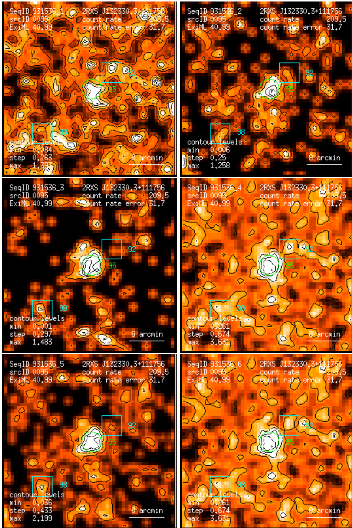
Figure 95: RASS 931536: detection 0095: band rate images, Gaussian filter: (1) PSPC channels 11 – 41, (2) 52 – 90, (3) 91 – 201, (4) 11 – 235, (5) 52 – 201, (6) 11 – 201. Broad band rates in counts/ks. Band rate contour levels in counts/ks/arcmin 2 .
