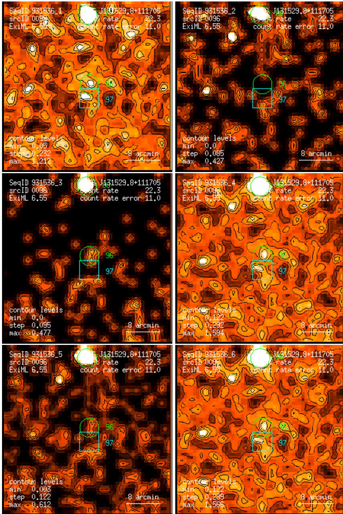
Figure 96: RASS 931536: detection 0096: band rate images, Gaussian filter: (1) PSPC channels 11 – 41, (2) 52 – 90, (3) 91 – 201, (4) 11 – 235, (5) 52 – 201, (6) 11 – 201. Broad band rates in counts/ks. Band rate contour levels in counts/ks/arcmin 2 .
