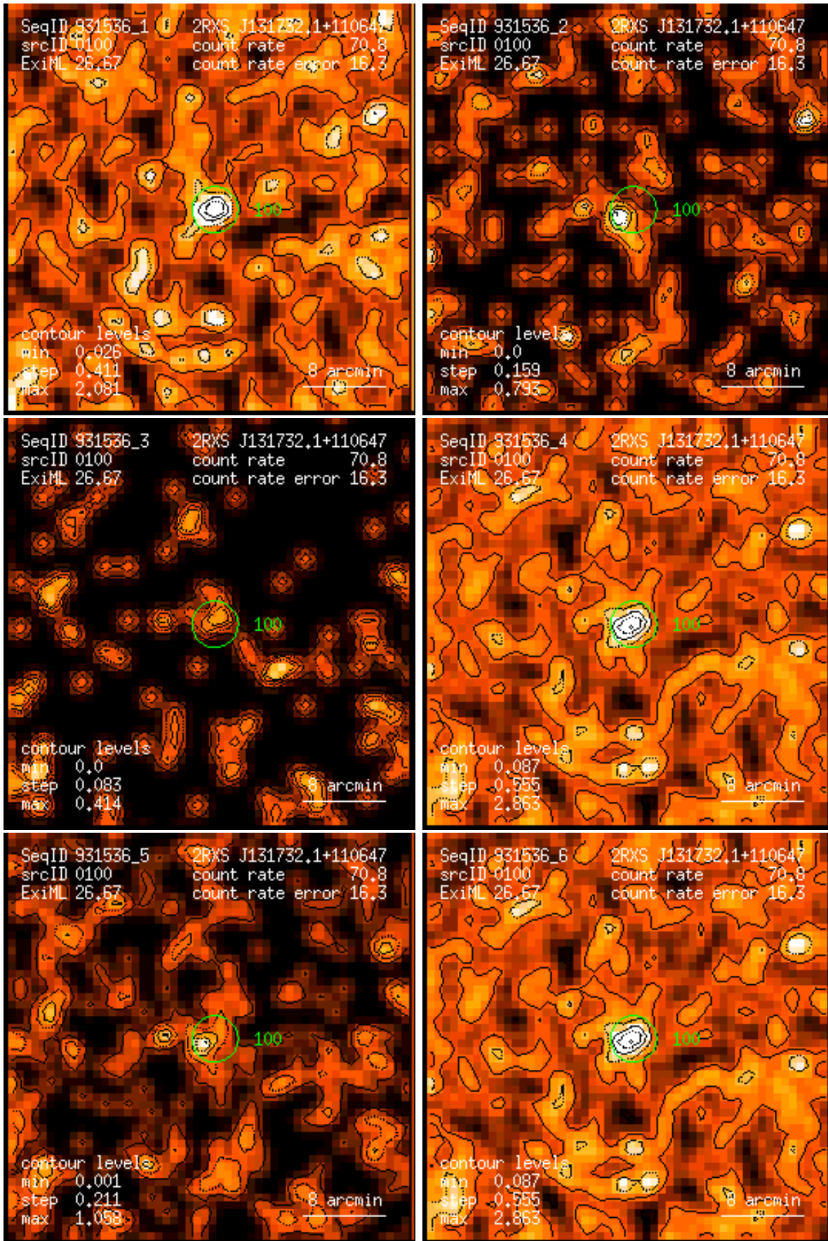
Figure 100: RASS 931536: detection 0100: band rate images, Gaussian filter: (1) PSPC channels 11 – 41, (2) 52 – 90, (3) 91 – 201, (4) 11 – 235, (5) 52 – 201, (6) 11 – 201. Broad band rates in counts/ks. Band rate contour levels in counts/ks/arcmin 2 .
