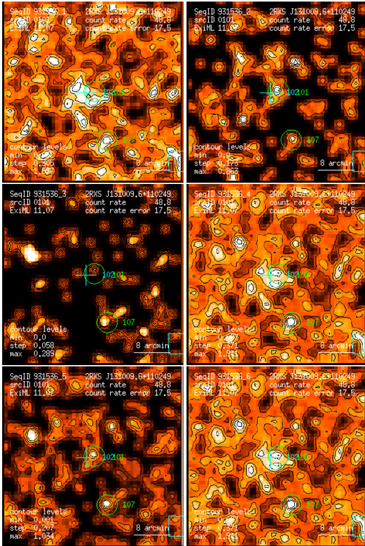
Figure 101: RASS 931536: detection 0101: band rate images, Gaussian filter: (1) PSPC channels 11 – 41, (2) 52 – 90, (3) 91 – 201, (4) 11 – 235, (5) 52 – 201, (6) 11 – 201. Broad band rates in counts/ks. Band rate contour levels in counts/ks/arcmin 2 .
