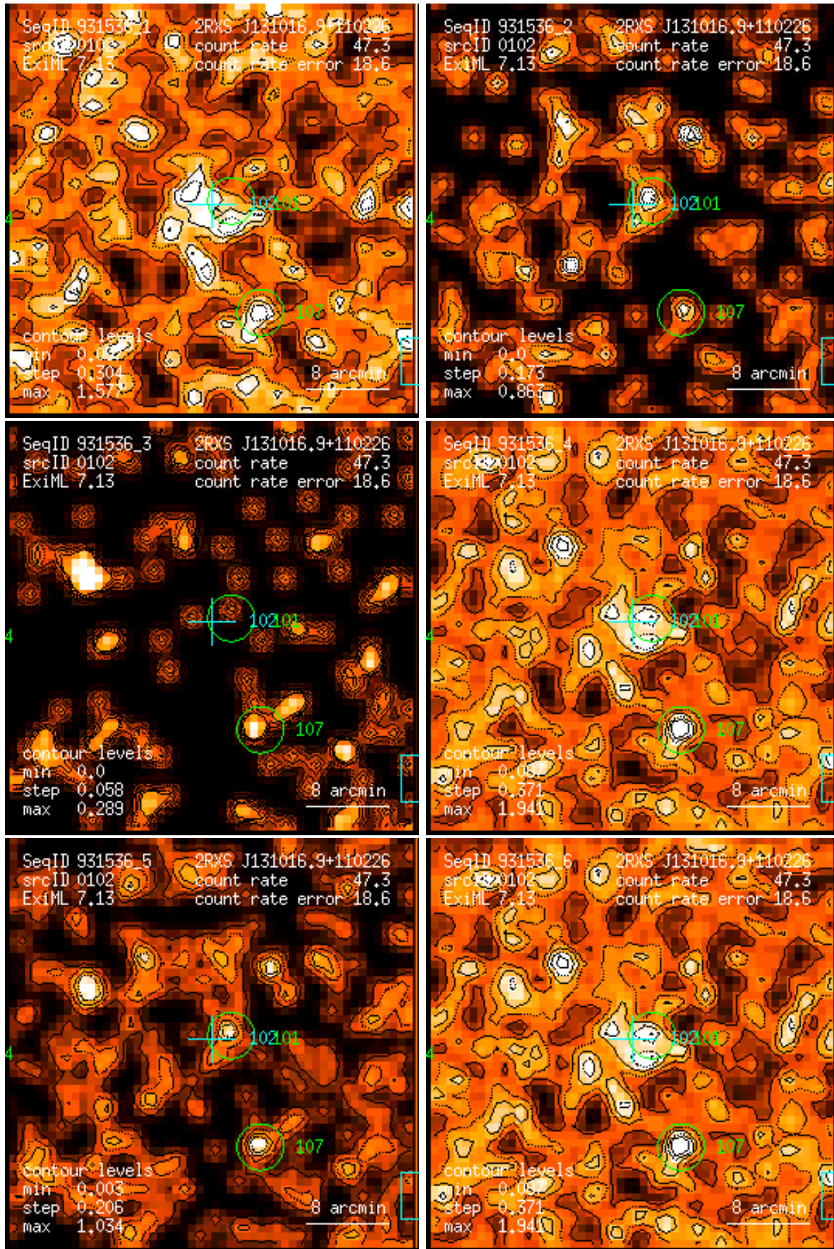
Figure 102: RASS 931536: detection 0102: band rate images, Gaussian filter: (1) PSPC channels 11 – 41, (2) 52 – 90, (3) 91 – 201, (4) 11 – 235, (5) 52 – 201, (6) 11 – 201. Broad band rates in counts/ks. Band rate contour levels in counts/ks/arcmin 2 .
