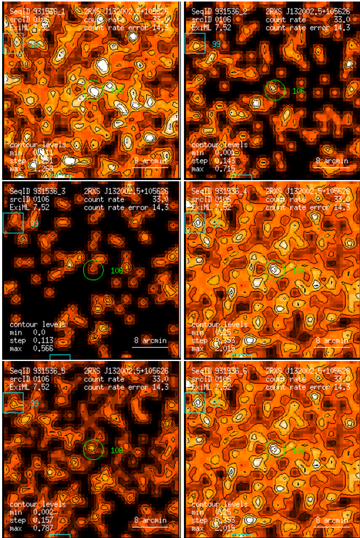
Figure 106: RASS 931536: detection 0106: band rate images, Gaussian filter: (1) PSPC channels 11 – 41, (2) 52 – 90, (3) 91 – 201, (4) 11 – 235, (5) 52 – 201, (6) 11 – 201. Broad band rates in counts/ks. Band rate contour levels in counts/ks/arcmin 2 .
