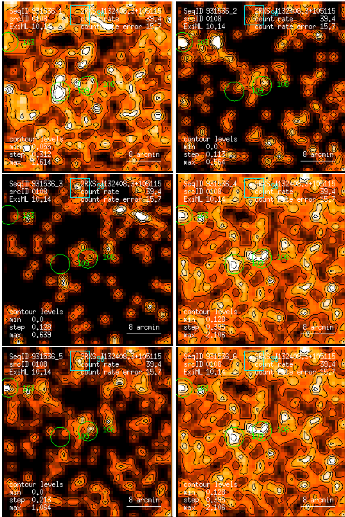
Figure 108: RASS 931536: detection 0108: band rate images, Gaussian filter: (1) PSPC channels 11 – 41, (2) 52 – 90, (3) 91 – 201, (4) 11 – 235, (5) 52 – 201, (6) 11 – 201. Broad band rates in counts/ks. Band rate contour levels in counts/ks/arcmin 2 .
