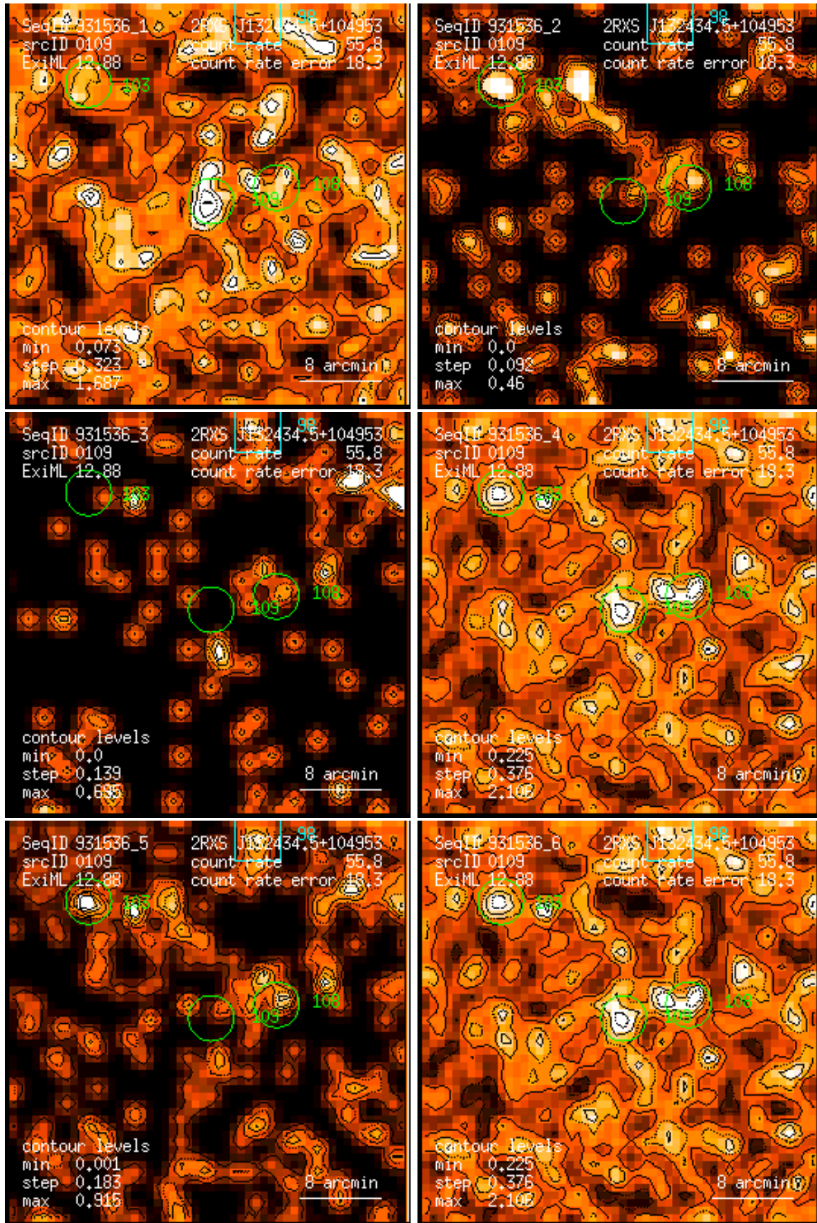
Figure 109: RASS 931536: detection 0109: band rate images, Gaussian filter: (1) PSPC channels 11 – 41, (2) 52 – 90, (3) 91 – 201, (4) 11 – 235, (5) 52 – 201, (6) 11 – 201. Broad band rates in counts/ks. Band rate contour levels in counts/ks/arcmin 2 .
