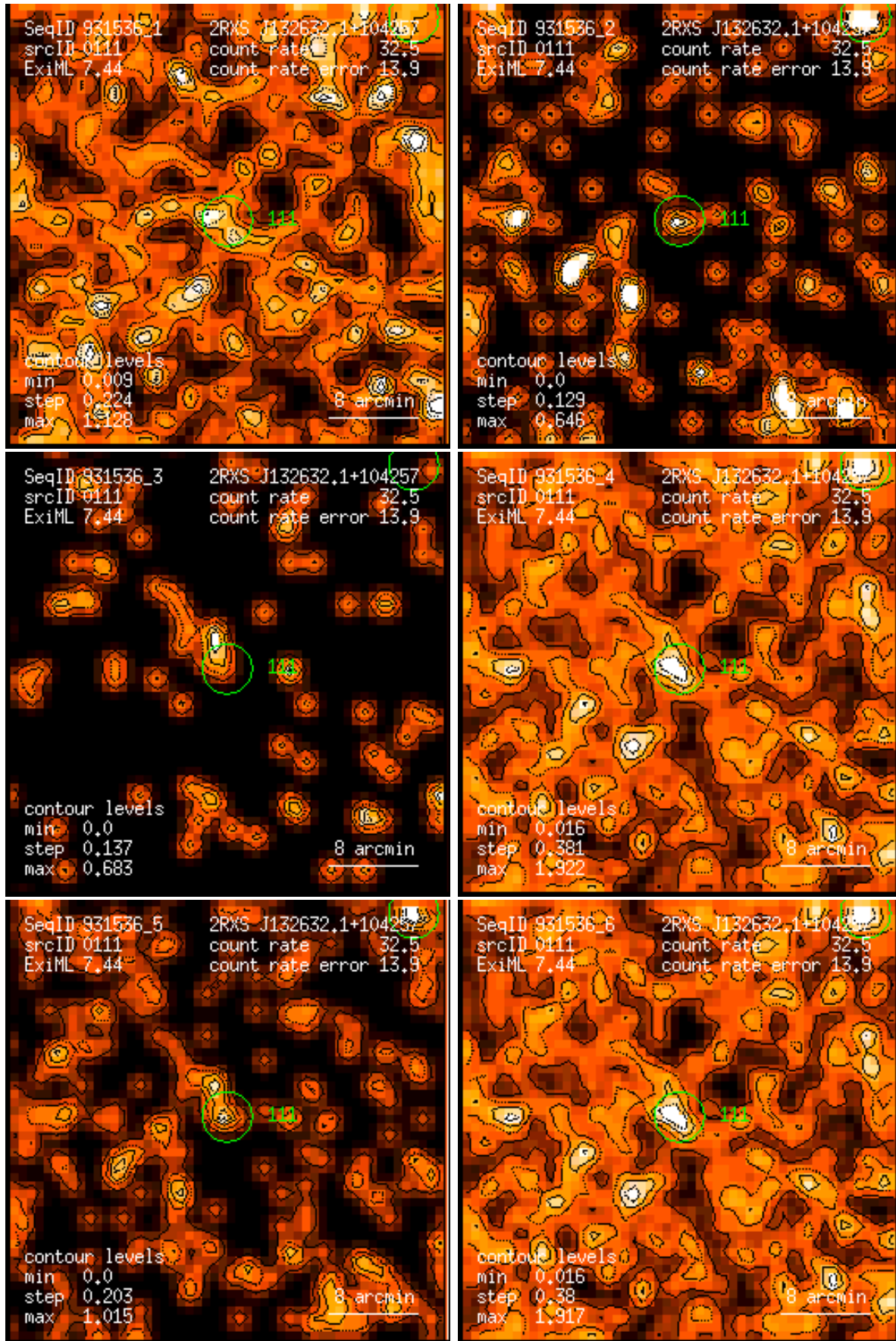
Figure 111: RASS 931536: detection 0111: band rate images, Gaussian filter: (1) PSPC channels 11 – 41, (2) 52 – 90, (3) 91 – 201, (4) 11 – 235, (5) 52 – 201, (6) 11 – 201. Broad band rates in counts/ks. Band rate contour levels in counts/ks/arcmin 2 .
