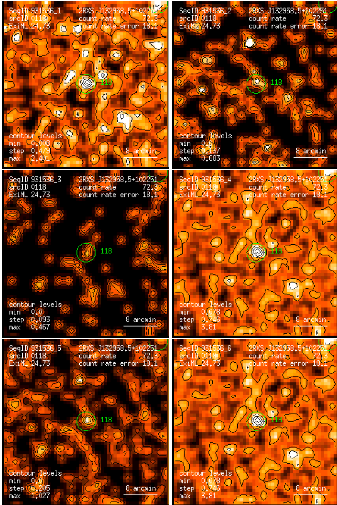
Figure 118: RASS 931536: detection 0118: band rate images, Gaussian filter: (1) PSPC channels 11 – 41, (2) 52 – 90, (3) 91 – 201, (4) 11 – 235, (5) 52 – 201, (6) 11 – 201. Broad band rates in counts/ks. Band rate contour levels in counts/ks/arcmin 2 .
