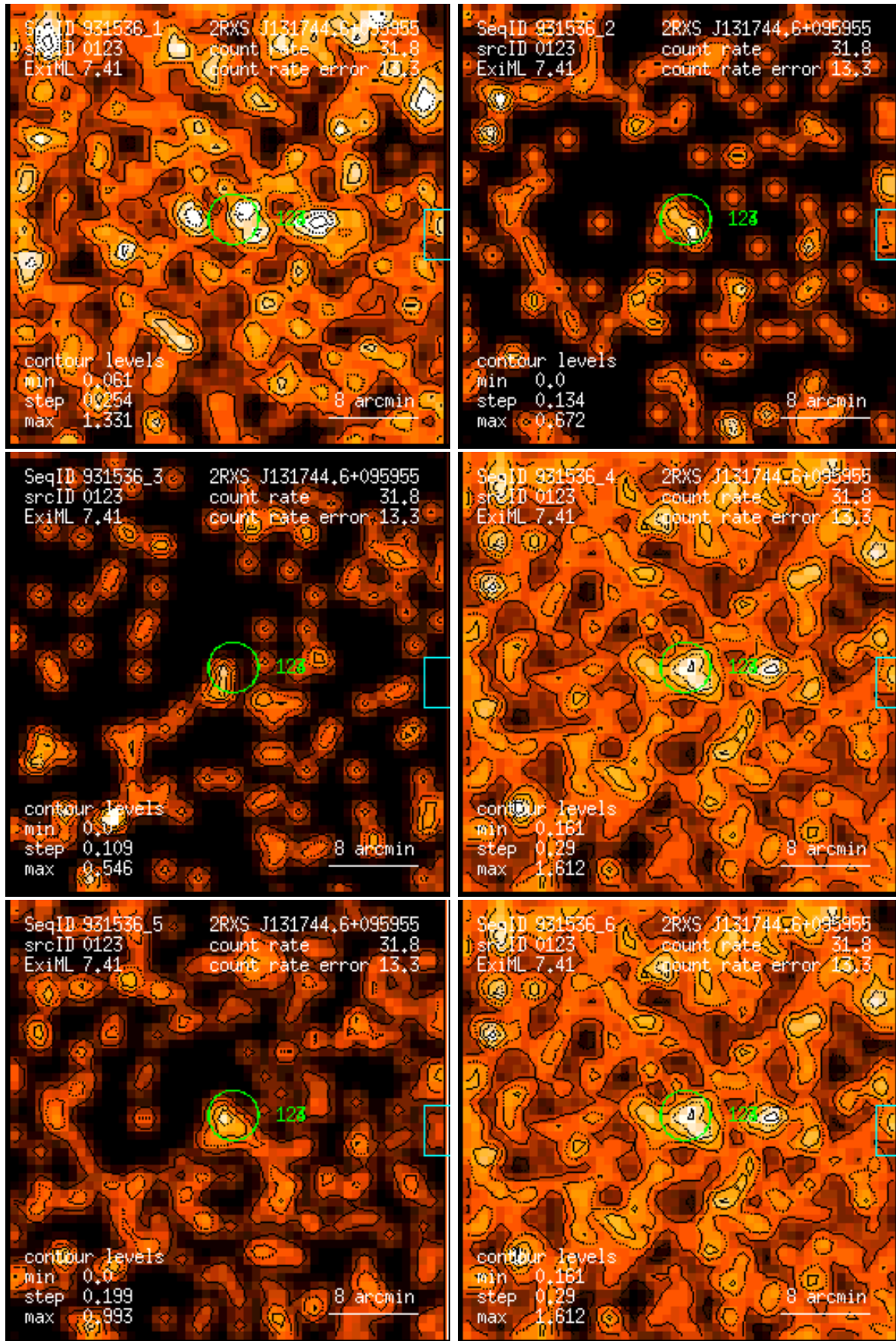
Figure 123: RASS 931536: detection 0123: band rate images, Gaussian filter: (1) PSPC channels 11 – 41, (2) 52 – 90, (3) 91 – 201, (4) 11 – 235, (5) 52 – 201, (6) 11 – 201. Broad band rates in counts/ks. Band rate contour levels in counts/ks/arcmin 2 .
