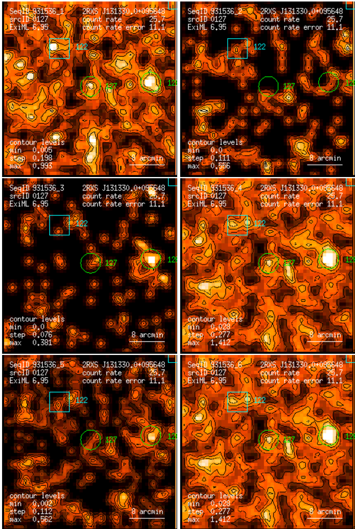
Figure 127: RASS 931536: detection 0127: band rate images, Gaussian filter: (1) PSPC channels 11 – 41, (2) 52 – 90, (3) 91 – 201, (4) 11 – 235, (5) 52 – 201, (6) 11 – 201. Broad band rates in counts/ks. Band rate contour levels in counts/ks/arcmin 2 .
