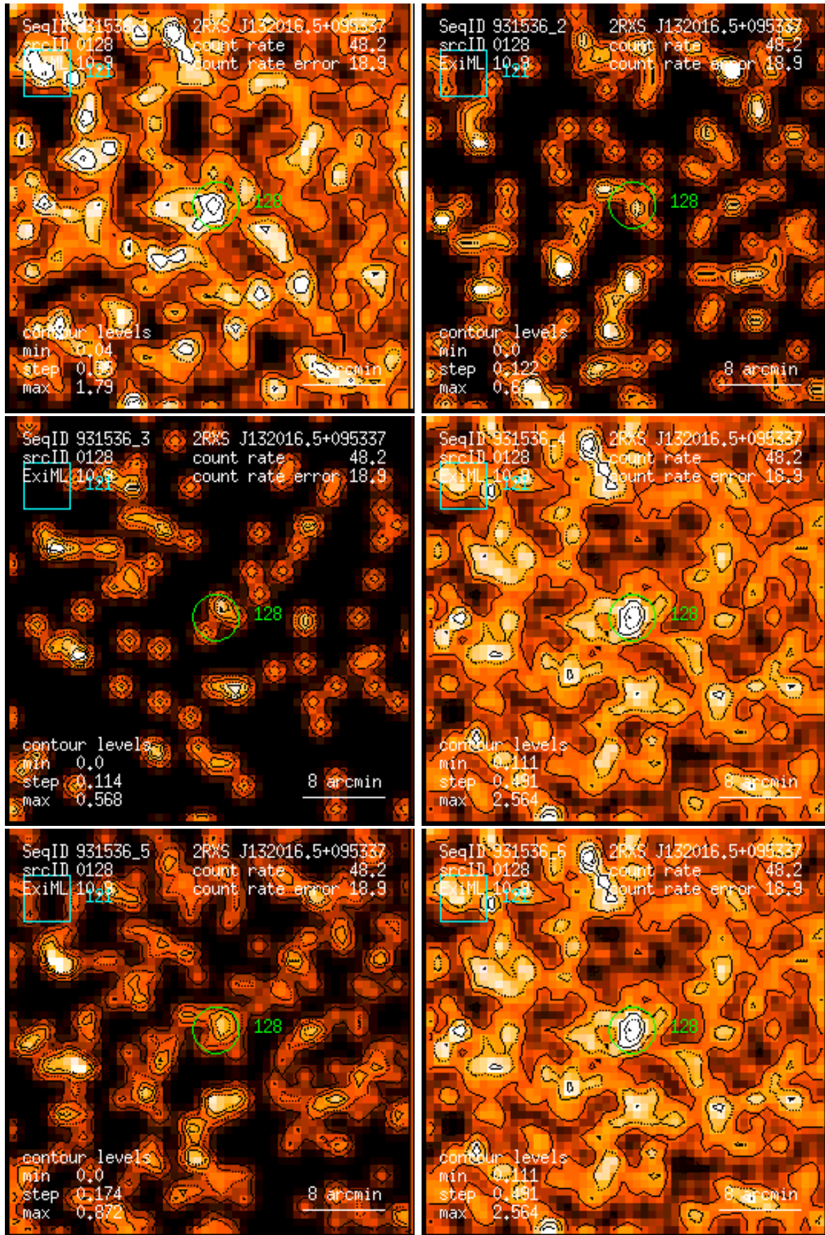
Figure 128: RASS 931536: detection 0128: band rate images, Gaussian filter: (1) PSPC channels 11 – 41, (2) 52 – 90, (3) 91 – 201, (4) 11 – 235, (5) 52 – 201, (6) 11 – 201. Broad band rates in counts/ks. Band rate contour levels in counts/ks/arcmin 2 .
