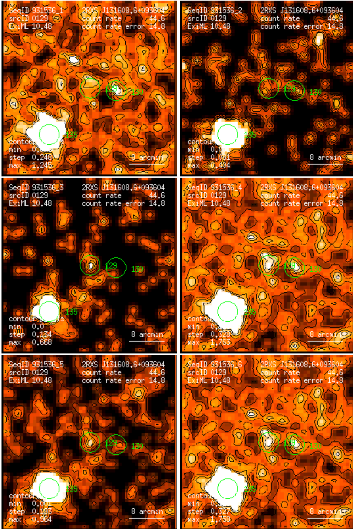
Figure 129: RASS 931536: detection 0129: band rate images, Gaussian filter: (1) PSPC channels 11 – 41, (2) 52 – 90, (3) 91 – 201, (4) 11 – 235, (5) 52 – 201, (6) 11 – 201. Broad band rates in counts/ks. Band rate contour levels in counts/ks/arcmin 2 .
