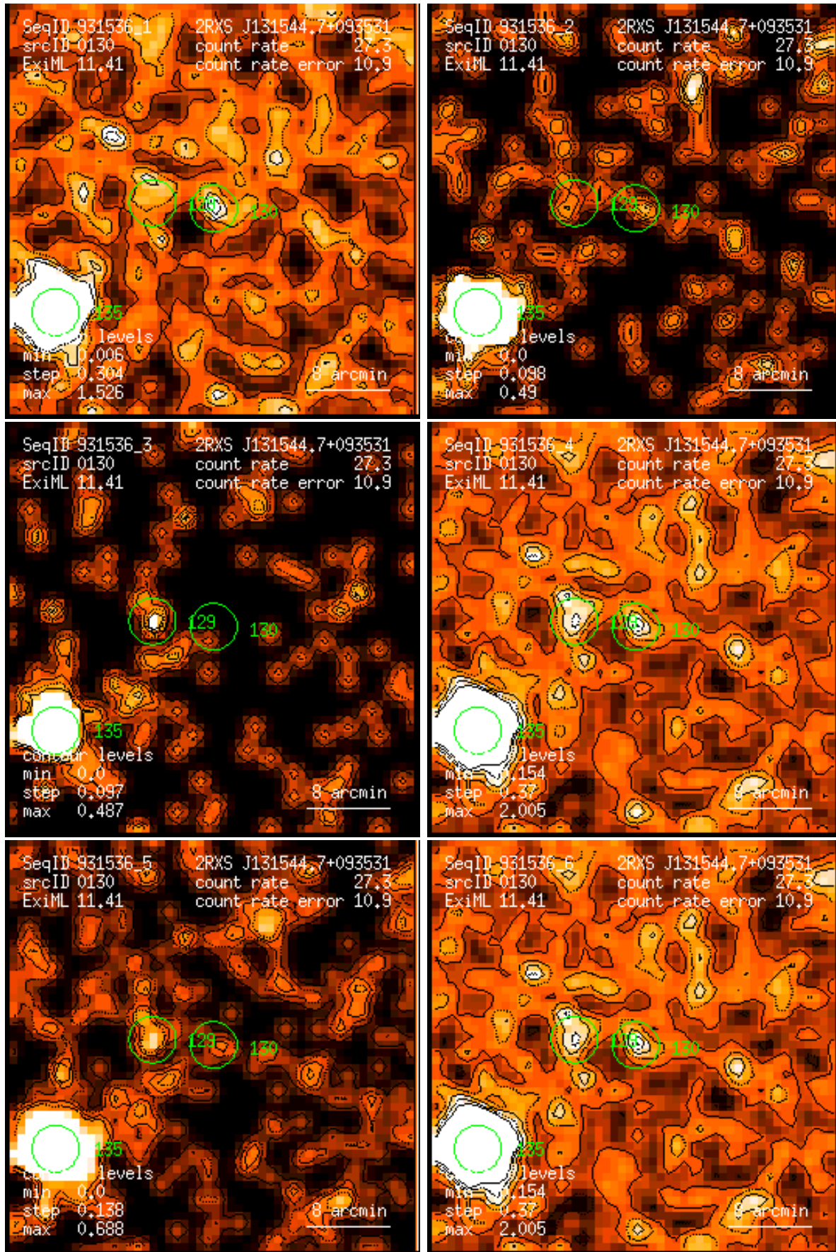
Figure 130: RASS 931536: detection 0130: band rate images, Gaussian filter: (1) PSPC channels 11 – 41, (2) 52 – 90, (3) 91 – 201, (4) 11 – 235, (5) 52 – 201, (6) 11 – 201. Broad band rates in counts/ks. Band rate contour levels in counts/ks/arcmin 2 .
