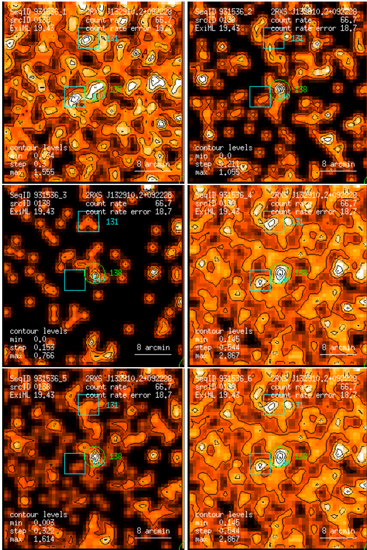
Figure 138: RASS 931536: detection 0138: band rate images, Gaussian filter: (1) PSPC channels 11 – 41, (2) 52 – 90, (3) 91 – 201, (4) 11 – 235, (5) 52 – 201, (6) 11 – 201. Broad band rates in counts/ks. Band rate contour levels in counts/ks/arcmin 2 .
