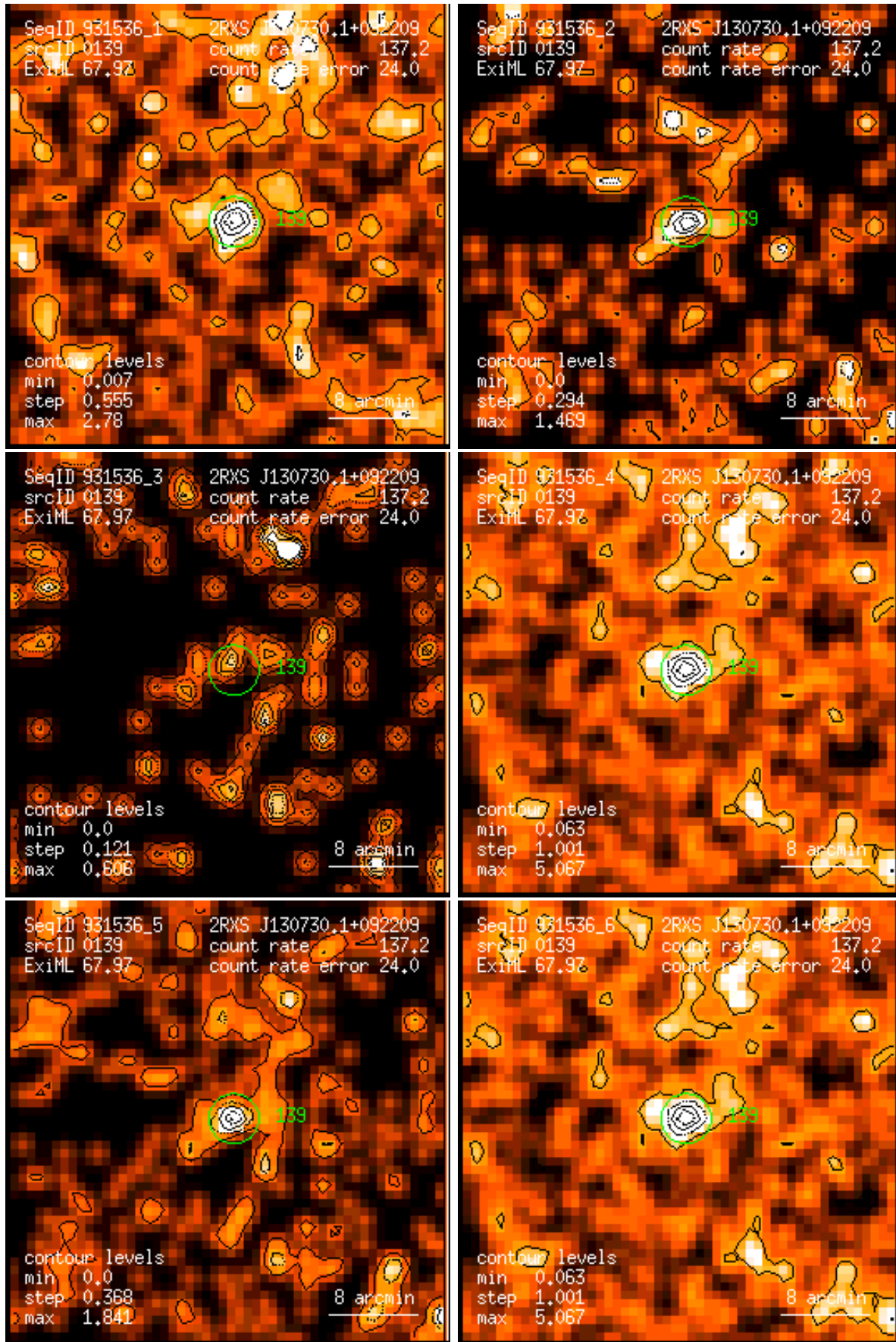
Figure 139: RASS 931536: detection 0139: band rate images, Gaussian filter: (1) PSPC channels 11 – 41, (2) 52 – 90, (3) 91 – 201, (4) 11 – 235, (5) 52 – 201, (6) 11 – 201. Broad band rates in counts/ks. Band rate contour levels in counts/ks/arcmin 2 .
