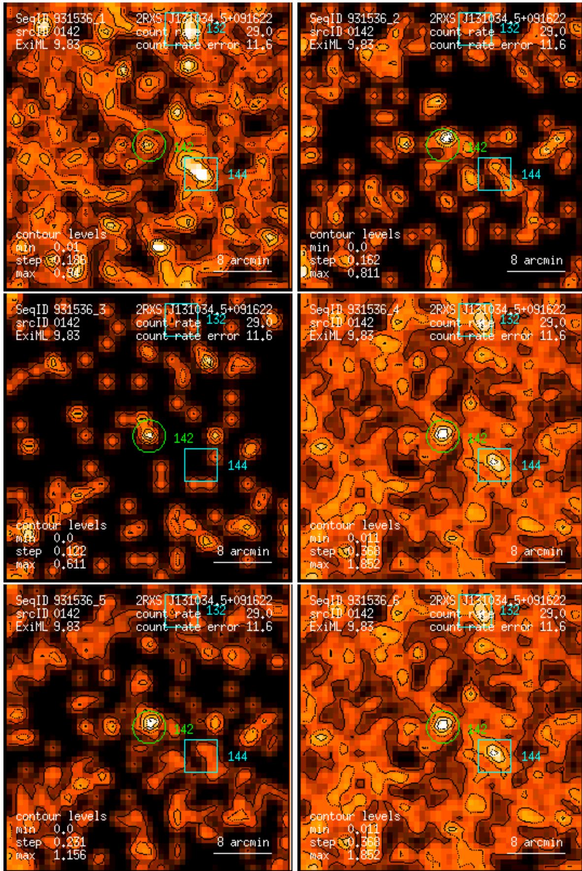
Figure 142: RASS 931536: detection 0142: band rate images, Gaussian filter: (1) PSPC channels 11 – 41, (2) 52 – 90, (3) 91 – 201, (4) 11 – 235, (5) 52 – 201, (6) 11 – 201. Broad band rates in counts/ks. Band rate contour levels in counts/ks/arcmin 2 .
