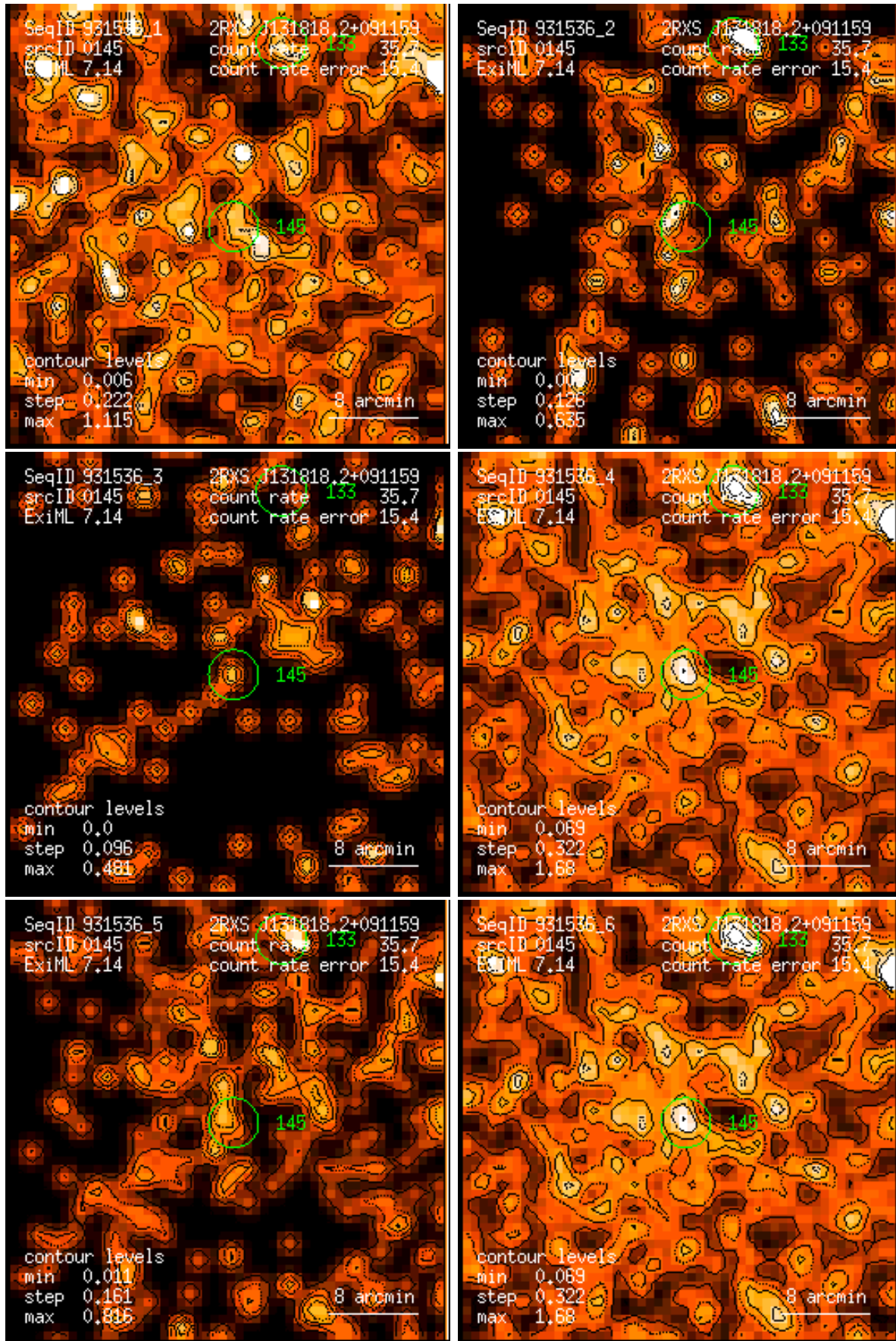
Figure 145: RASS 931536: detection 0145: band rate images, Gaussian filter: (1) PSPC channels 11 – 41, (2) 52 – 90, (3) 91 – 201, (4) 11 – 235, (5) 52 – 201, (6) 11 – 201. Broad band rates in counts/ks. Band rate contour levels in counts/ks/arcmin 2 .
