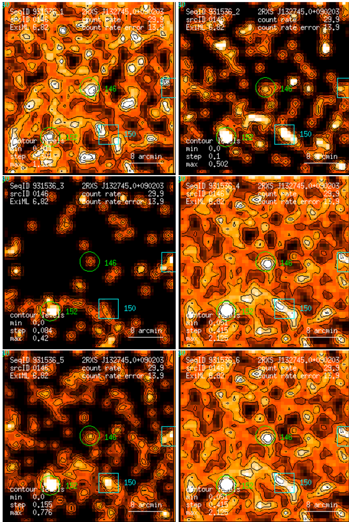
Figure 146: RASS 931536: detection 0146: band rate images, Gaussian filter: (1) PSPC channels 11 – 41, (2) 52 – 90, (3) 91 – 201, (4) 11 – 235, (5) 52 – 201, (6) 11 – 201. Broad band rates in counts/ks. Band rate contour levels in counts/ks/arcmin 2 .
