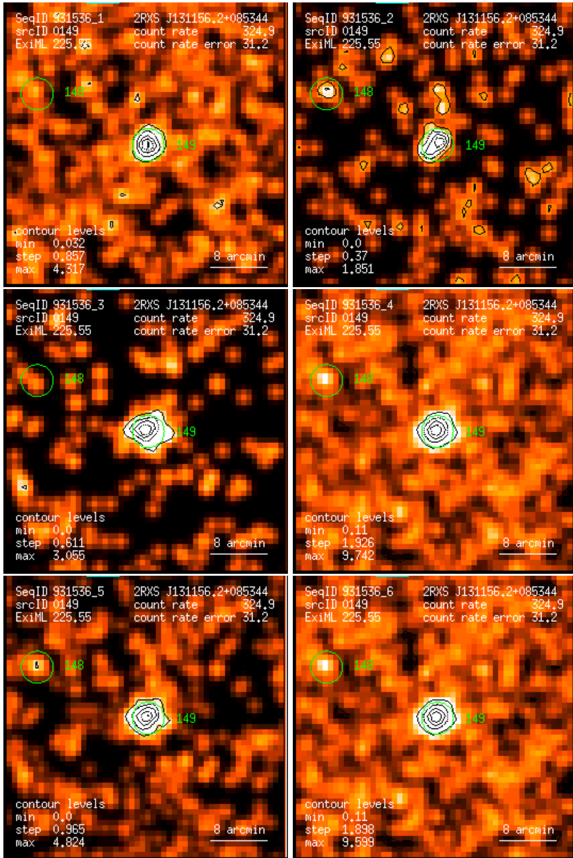
Figure 149: RASS 931536: detection 0149: band rate images, Gaussian filter: (1) PSPC channels 11 – 41, (2) 52 – 90, (3) 91 – 201, (4) 11 – 235, (5) 52 – 201, (6) 11 – 201. Broad band rates in counts/ks. Band rate contour levels in counts/ks/arcmin 2 .
