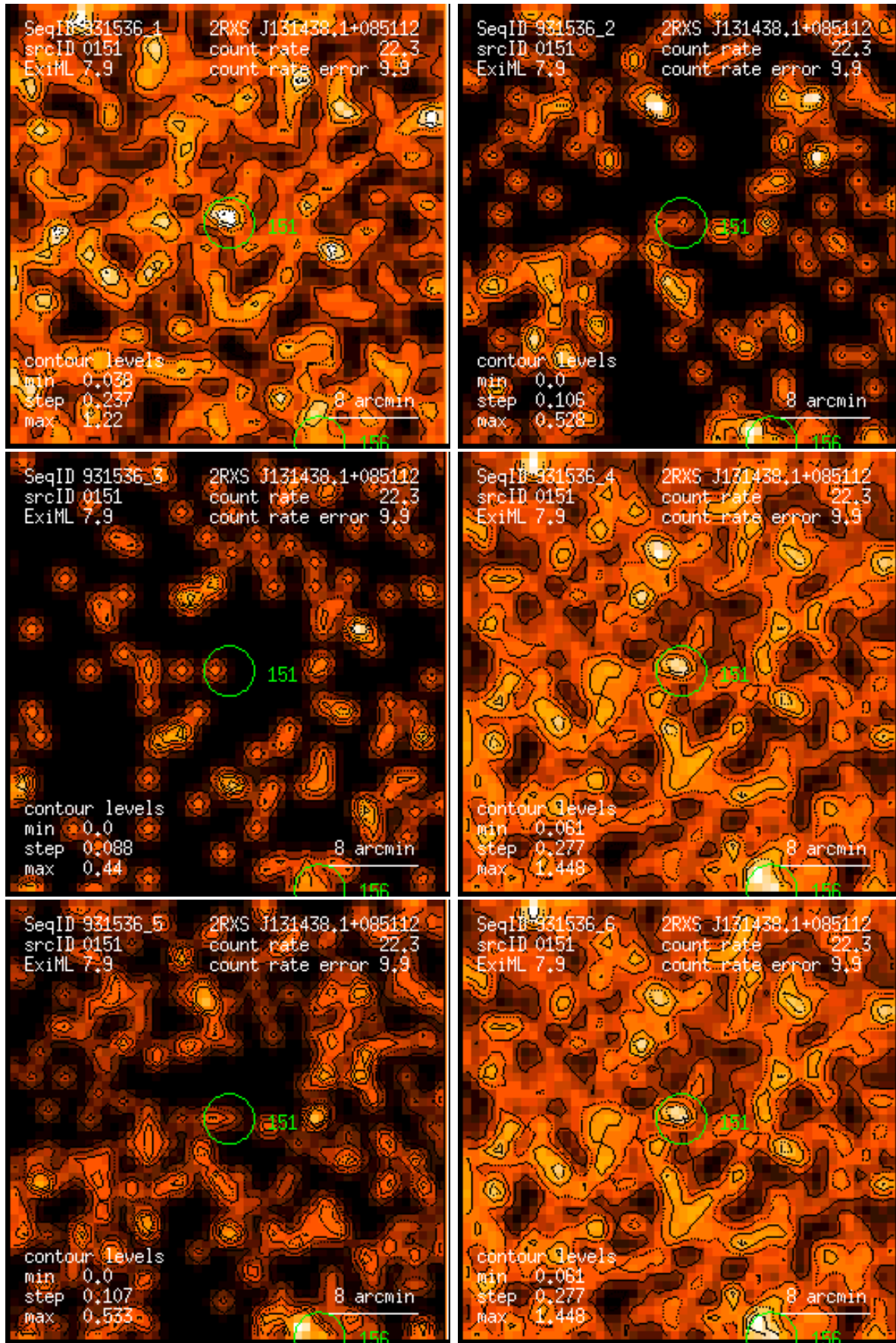
Figure 151: RASS 931536: detection 0151: band rate images, Gaussian filter: (1) PSPC channels 11 – 41, (2) 52 – 90, (3) 91 – 201, (4) 11 – 235, (5) 52 – 201, (6) 11 – 201. Broad band rates in counts/ks. Band rate contour levels in counts/ks/arcmin 2 .
