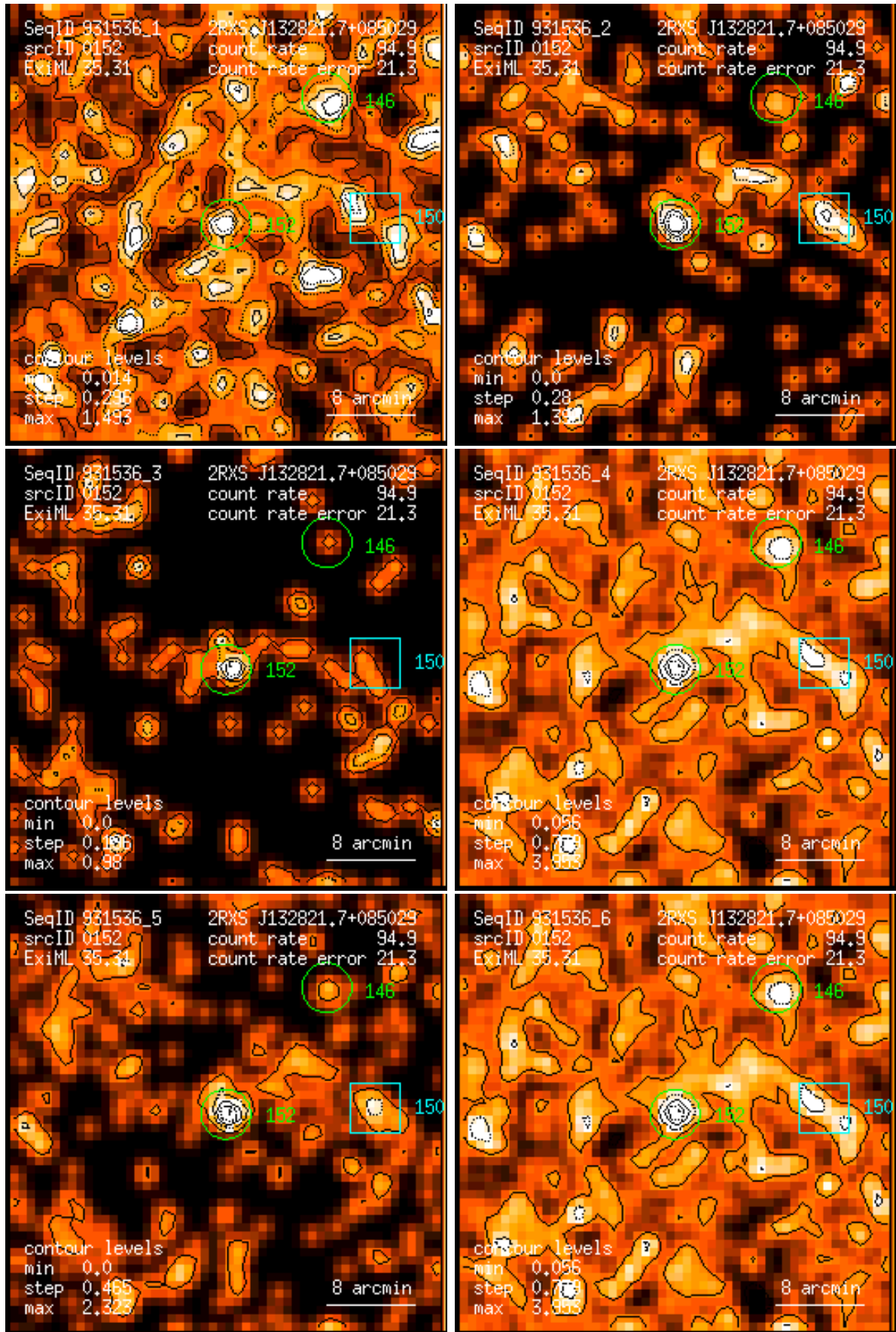
Figure 152: RASS 931536: detection 0152: band rate images, Gaussian filter: (1) PSPC channels 11 – 41, (2) 52 – 90, (3) 91 – 201, (4) 11 – 235, (5) 52 – 201, (6) 11 – 201. Broad band rates in counts/ks. Band rate contour levels in counts/ks/arcmin 2 .
