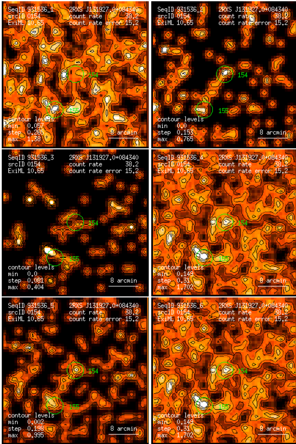
Figure 154: RASS 931536: detection 0154: band rate images, Gaussian filter: (1) PSPC channels 11 – 41, (2) 52 – 90, (3) 91 – 201, (4) 11 – 235, (5) 52 – 201, (6) 11 – 201. Broad band rates in counts/ks. Band rate contour levels in counts/ks/arcmin 2 .
